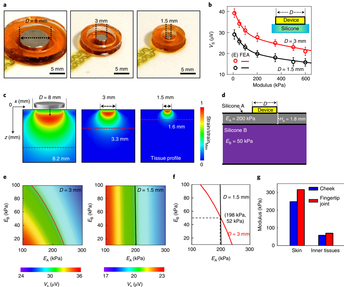
Fig. 4 | Designs for modulus sensing and depth profiling of multilayer samples. a, Photographs of devices with various sensing areas. b, Simulated (FEA, line) and measured (E, circles) V_s values for systems with different dimensions as a function of the elastic modulus for artificial skin samples. D represents the sensing diameter of the EMM sensor. Error bars correspond to the standard deviation for ten measurements with a given device with different D . c, Normalized FEA results for distributions of strain throughout the tissue structure with a modulus of 200 kPa, shown in the cross-sectional profile during actuator vibration, with different D . z is the depth into the tissue and x corresponds to the direction along the surface. The effective saturation depths decrease with decreasing D from 8 mm to 1.3 mm. d, Schematic illustration of a bilayer structure that approximates the skin/tissue system, with modulus values of 200 kPa and 50 kPa, and with thicknesses of 1.8 mm and >>1 cm, for the top and bottom layers, respectively. e,f, FEA modelling to determine the modulus of each layer in the bilayer structure from measurements using EMM sensors with different D ( e ), yielding simulation results for E_A and E_B ( f ). g, Simulated results of moduli for the skin and underlying tissues of the cheek and fingertip joint of a human participant.
