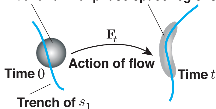
Figure 1. Schematic of the effect of the co-dimension 1 manifold, corresponding to the trench of the attraction rate, s_1 , at an initial time, on a small parcel of phase space. The image of the trench under the time- t flow map, F_t , is also shown.
