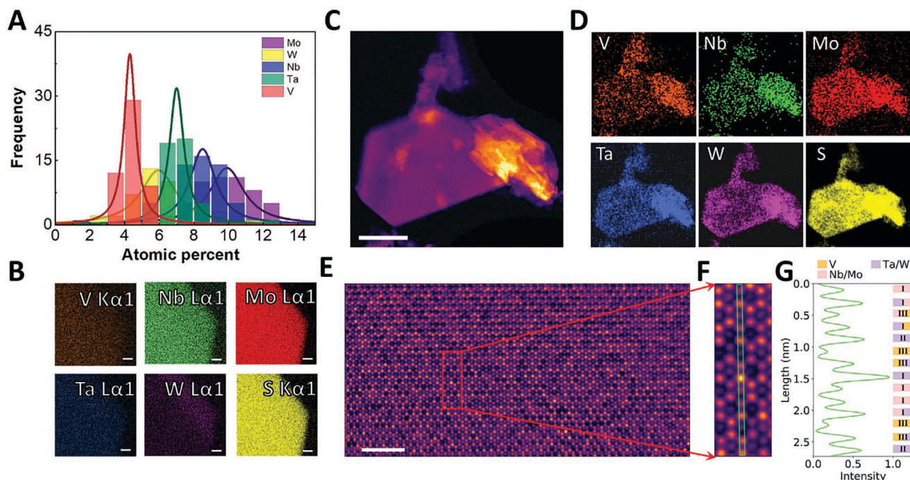
Figure 2. Experimental verification of successful synthesis of the TMDC HEA (Mo,W,V,Nb,Ta). A) Histogram TM stoichiometries from 60 synthesized flakes from SEM-EDX data. B) Elemental-mapping EDS data showing a homogeneous spatial distribution of each TM in a representative (Mo, W, V, Nb, Ta) flake. C) STEM-HAADF image showing a typical high entropy TMDC flake. D) EDS chemical maps showing V, Nb, Mo, Ta, W, and S distribution for the flake shown in (C). E) STEM-HAADF image of a flake, where the highlighted region (red box) shows the [001] projection of a typical TMDC structure. F) Atomic-resolution STEM-HAADF image showing local variations in the intensity of atomic columns due to varying composition of cations. G) Intensity profile of the region illustrated in (F) as a green box, where the legends correspond to the predominant elements in each atomic column. The scale bars correspond to 100 nm for (C) and 2 nm for (E).
