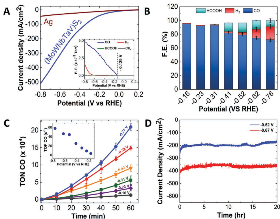
Figure 3. Experimental \text{CO}_2\text{RR} catalysis results for (Mo, W, V, Nb, Ta). A) The current density of (Mo, W, V, Nb, Ta) and Ag nanoparticles plotted against V versus RHE using LSV with simultaneous measurements of partial pressure of gaseous products in the inset. B) Faradaic efficiency (F.E.) of \text{CO} , \text{H}_2 and \text{HCOOH} from chronoamperometry experiments using (Mo, W, V, Nb, Ta) NFs at different potentials. The error bars represent the standard deviation of three experiments. C) Turn over numbers (TON) of \text{CO} formation over the course of an hour at various voltages with the turnover frequency (TOF) of the CA inset. D) Long-term chronoamperometry experiments (20 h) at 2 different potentials. Potentials in (C) and (D) are based on RHE.
