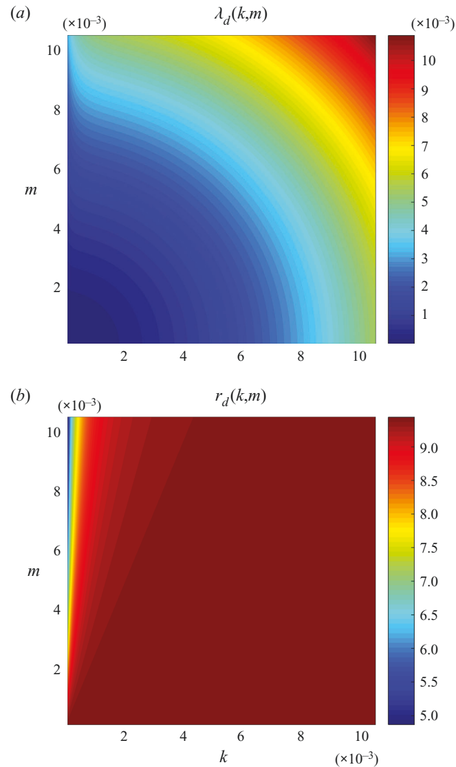
FIGURE 10. The wave decay rate ( \lambda_d ) and the attenuation ratio ( r_d ) realized in the diffusive case are plotted as functions of wavenumbers ( k, m ) in (a) and (b) respectively.
