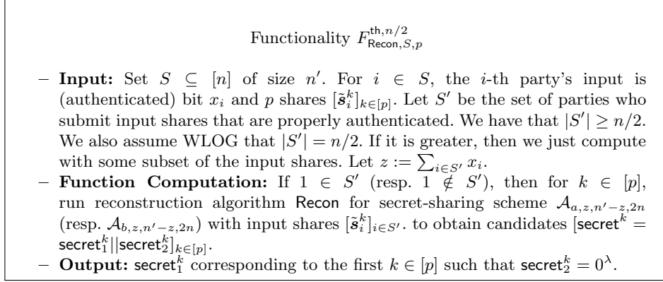
Fig. 2. RECONSTRUCTION FUNCTIONALITY WITH RESPECT TO p SETS OF SECRET SHARES.
