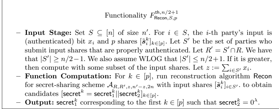
Fig. 4. RECONSTRUCTION FUNCTIONALITY WITH RESPECT TO p SETS OF SECRET SHARES.
