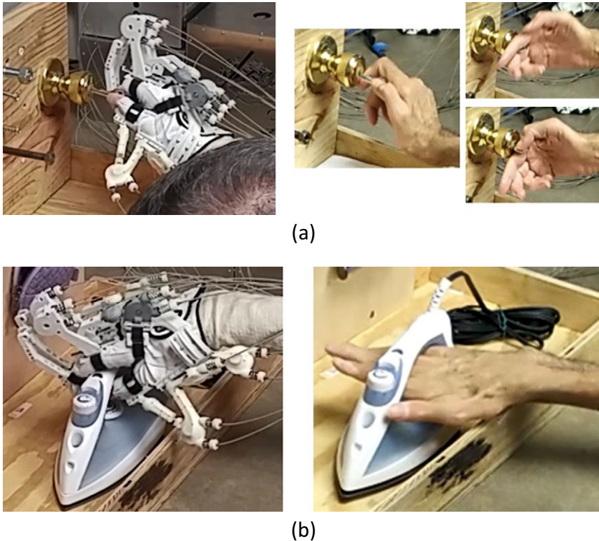
Figure 12. Hand poses with Maestro (left) and without Maestro (right) during (a) pick up key, put into Yale-lock and turn 90° and (b) lift iron over edge for S01.
