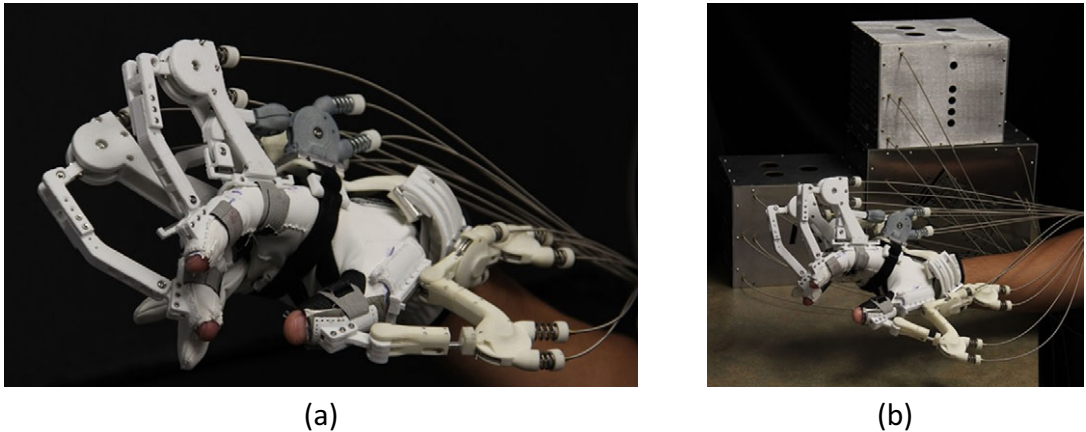
Figure 1. Developed hand exoskeleton (a) Maestro and (b) overall system for Maestro .
