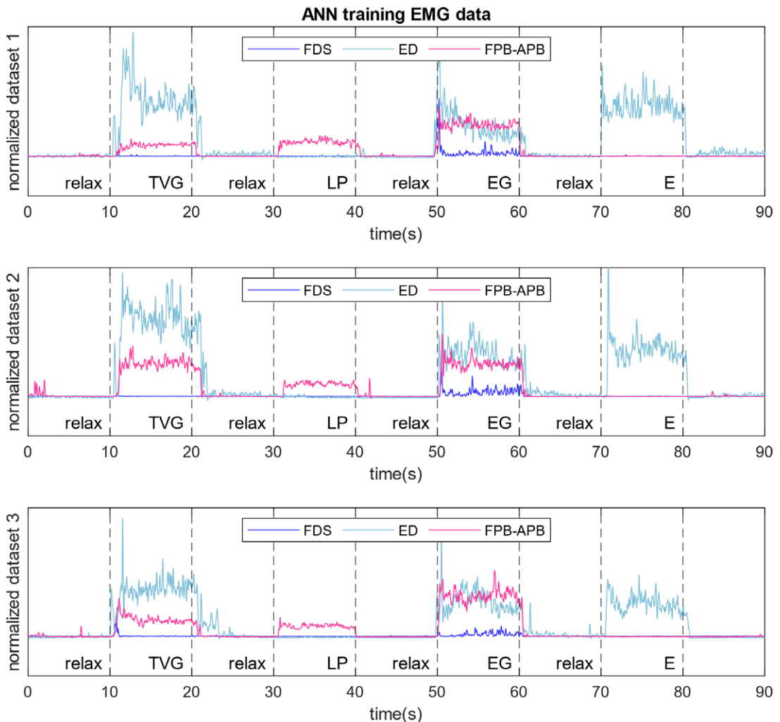
Figure 5. Postprocessed signals extracted from three sensors during training of ANN for hand pose classification. Targeted muscles signals are from FDS, ED, and a combination of FPB and APB. The differences in signal trends between different hand poses, and the similarity of signals of a specific hand pose between trials make it possible to perform intention recognition through the ANN.
