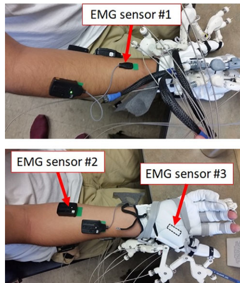
Figure 4. Three wireless sEMG sensors were utilized to identify the intentions of the SCI patients. Three sensors detected the flexion of the fingers, extension of the fingers, and thumb flexion and abduction.
