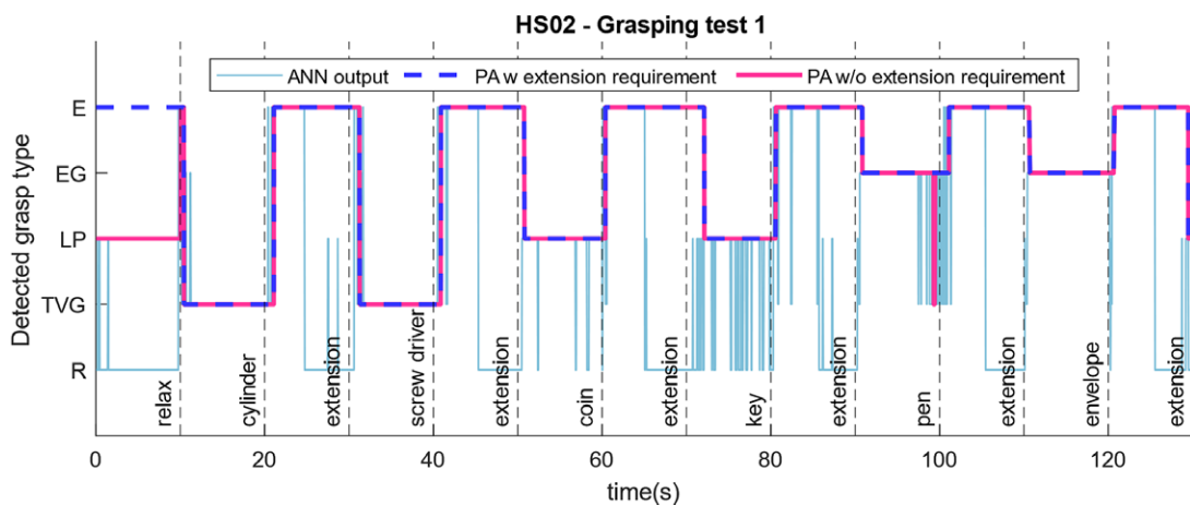
Figure 11. Reliability of the probabilistic approach for selecting the correct hand pose command for the robot shown in two different tests for the second healthy subject (HS02).
