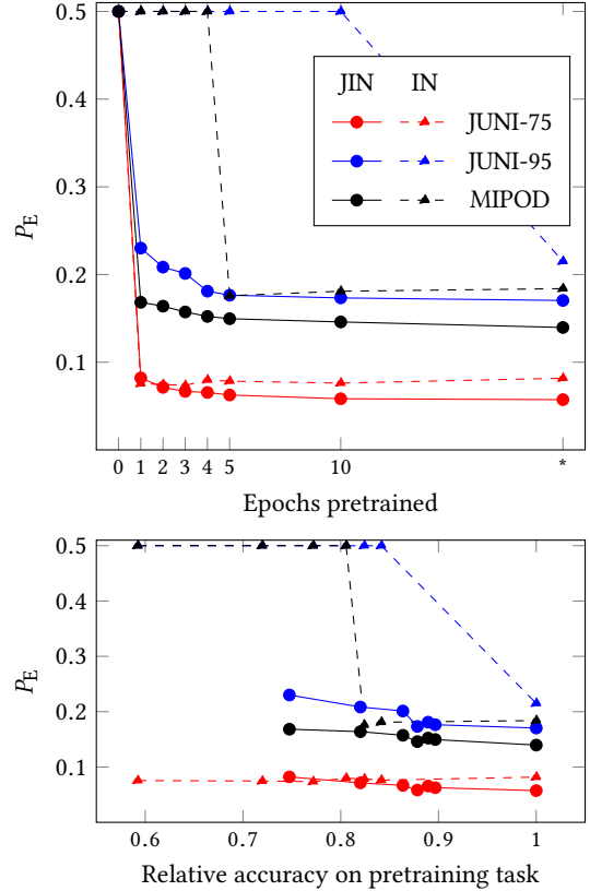
Figure 2: SRNet’s detection error P_E at 0.4 bpnzac on BOSS-base1.01+BOWS2. Top: P_E vs. the number of pretrained epochs; IN was pretrained for twice as many epochs because its training set is roughly twice smaller. The superscript * corresponds to the best checkpoint on the pretraining task, which is 57 for JIN and 98 for IN. Bottom: P_E as a function of the relative accuracy w.r.t. the best checkpoint on the pretraining task.
