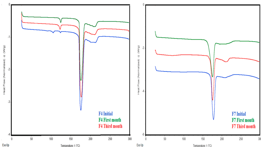
Fig. 8. DSC thermograms of 1:1 theophylline nicotinamide 170 °C (F4) and 1:1 theophylline nicotinamide with 5% Kollidon® VA-64 (F7) extrudates on the first day, first month, and third month at 40 (\pm 2) ^\circ\text{C} and 75 (\pm 5) \% \text{RH} .
