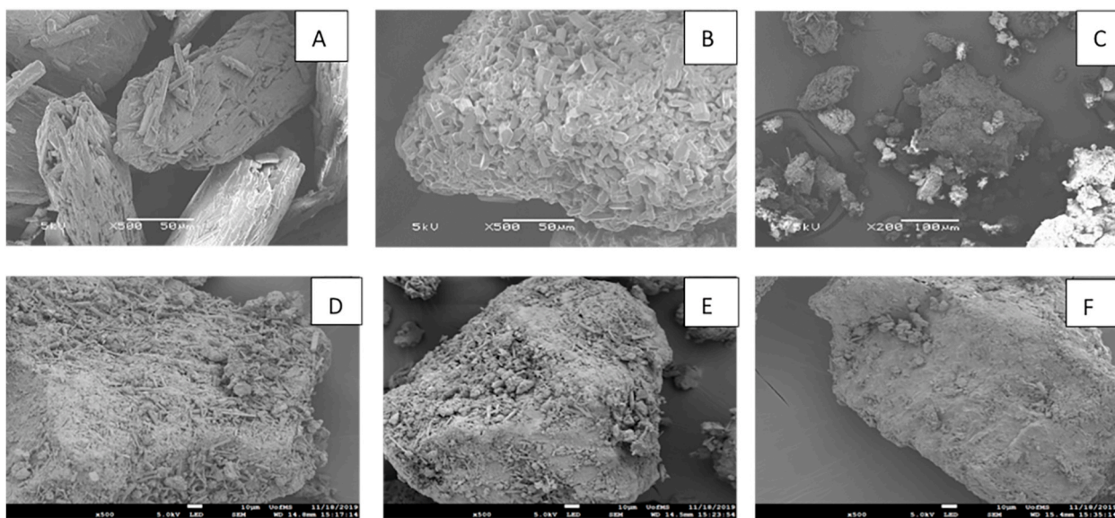
Fig. 6. Scanning electron microscopy (SEM) images of (A) pure theophylline, (B) pure nicotinamide, (C) 1:1 Theophylline Nicotinamide 170 °C (F4) extrudates, (D) 1:1 Theophylline Nicotinamide with 5% HPMCAS-MG (F5), (E) 1:1 Theophylline Nicotinamide with 5% PEO (F6), and (F) 1:1 Theophylline Nicotinamide with 5% Kollidon® VA-64 (F7).
