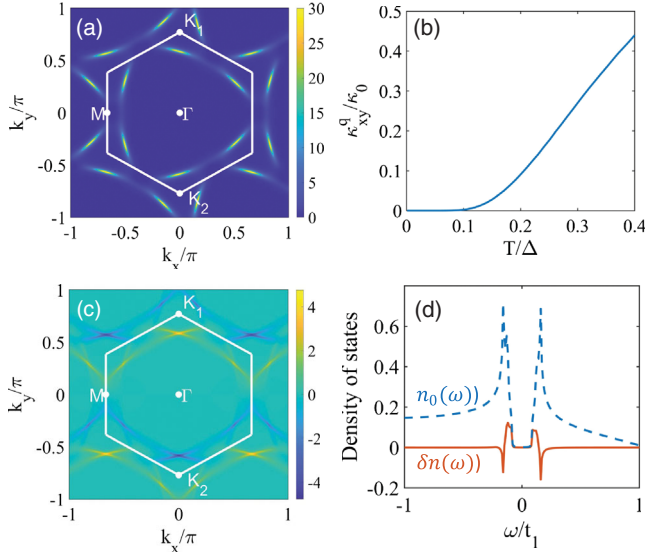
FIG. 1. (a) Berry curvatures of the tight-binding model for twisted-bilayer graphene with d_{x^2-y^2} and id_{xy} superconducting gaps. (b) The quasiparticle thermal Hall conductivity as a function of temperature. Berry-curvature modifications to the momentum space (c) and local (d) density of states with a constant supercurrent \nabla_r\theta = (\sqrt{2}\pi/10)\hat{x} . In (d) only the result for one of the two bands at the Fermi surface is plotted (solid line). The conventional density of states n_0(\omega) is demonstrated for comparison. Model parameters are taken as t_2/t_1 = 0.05 , t_3/t_1 = 0.2 , \mu = -0.9t_1 , and \Delta/t_1 = 0.1 .
