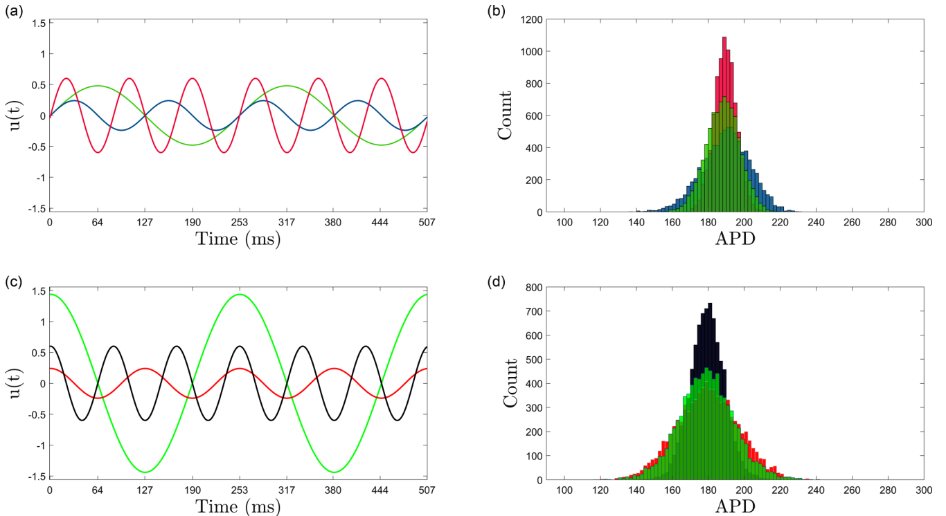
FIG. 7. Green lines in panels (A) and (C) represent the baseline stabilizing stimulus u_1(t) (in \mu\text{A}/\text{cm}^2 ) as described in the procedure from Sec. III E 2. Green bars in panels (B) and (D) show the respective histograms of the APDs. Black, red, and blue lines in panels (A) and (C) show stimuli u_2(t) - u_1(t) , highlighting the additional inputs added to u_1(t) . Histograms of corresponding color are shown in panels (B) and (D). Differences between the resulting variances of the measured action potentials are then used to infer information about the shape of C(\theta) .
