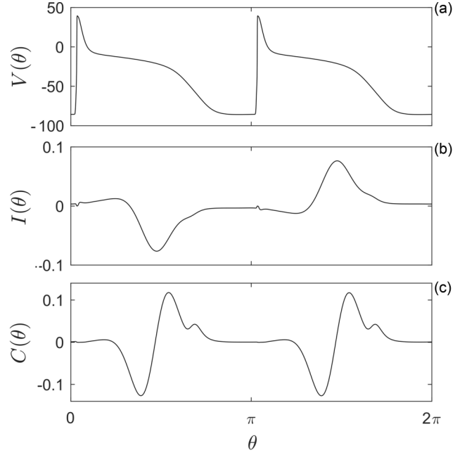
FIG. 2. The panels above show relevant terms from the reduction Eq. (6). The Noble model from Appendix A is considered with a pacing rate of 290 ms. As described in the text, two action potentials are used to define the periodic orbit so that the resulting Floquet multipliers are positive. Panel (A) shows the voltage trace on the periodic orbit, with panels (B) and (C) giving the corresponding values of I(\theta) and C(\theta) , respectively.
