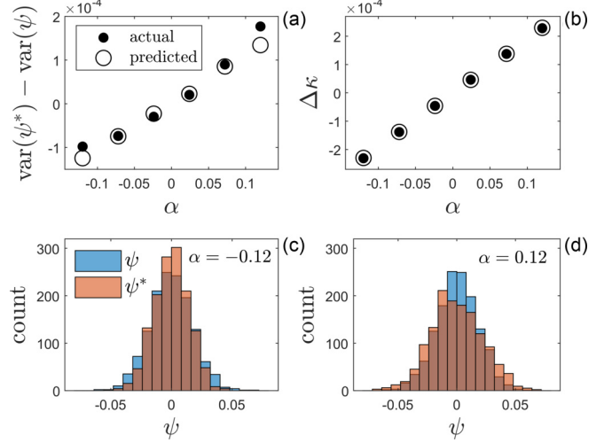
FIG. 3. Numerical confirmation of the derived relationships between changing Floquet multipliers and the variance of the resulting isostable coordinates for simulations of Eqs. (16) and (23). Black dots in panel (A) show how the variance of the isostable coordinates changes when input u(t) = \alpha \sin(8\pi t/T) is applied. Predictions computed according to Eq. (25) are shown as open circles. Histograms of the measurements of the isostable coordinates obtained from simulations of Eqs. (16) and (23) are shown in Panels (C) and (D) providing a visual representation of the change in variance that results when sinusoidal input is applied. Note that overlapping regions of the histograms in panels (C) and (D) appear brown.
