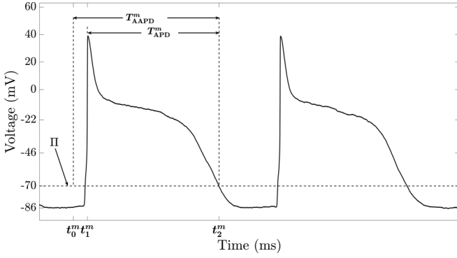
FIG. 4. While the APD, defined in Eq. (28) is a more natural experimental definition, both t_1^m and t_2^m are random variables, which would complicate the analysis below. By contrast, the AAPD defined in Eq. (29) consists of only one random variable (since t_0^m is deterministic). In practice, since \text{var}(t_1^m - t_0^m) is small, the difference between the variance of the APDs and AAPDs is negligible. The voltage threshold, \Pi , defines a Poincaré section that is used to calculate APDs.
