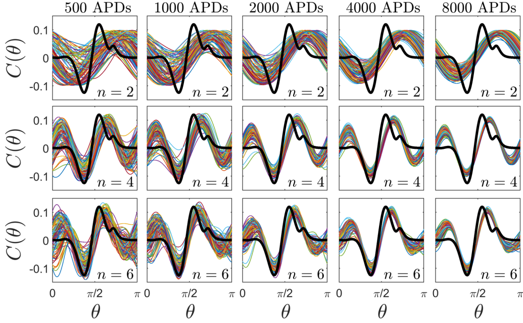
FIG. 8. Results from implementing the proposed strategy from Sec. III E 2 for estimating C(\theta) from the reduced equations of the form Eq. (6) associated with an unstable periodic orbit. Each panel shows 100 independent estimates of C(\theta) (colored lines) using the indicated number of APDs to estimate the required APD variances according to the Fourier series expansion C(\theta)/\mu = a_0/2 + \sum_{k=0}^n [b_k \sin(2\pi kt/T) + a_n \cos(2\pi kt/T)] . The magnitudes of the resulting plots are appropriately normalized to provide visual comparisons with the exact solutions. The black lines in each panel show the exact value of C(\theta) calculated numerically from the model equations using methods described in Ref. [18]. Taking more terms of the Fourier series expansion (i.e., with n larger than 6) only yields small differences in the resulting values of C(\theta) and these results are not shown.
