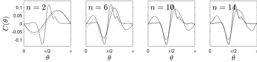
FIG. 5. Illustration of the proposed strategy for estimating C(\theta) of the reduced model Eq. (6) for a stable entrained orbit. The gray lines in each panel show the exact value of C(\theta) calculated directly from the model equations using methods described in Ref. [18]. Black lines in each panel show the data-driven approximation of C(\theta)/\mu = a_0/2 + \sum_{k=0}^n [b_k \sin(2\pi kt/T) + a_n \cos(2\pi kt/T)] for the indicated value of n . The coefficients of the Fourier series expansion are determined using the strategy detailed in Sec. III E 1. Dashed lines show the first n Fourier modes of the exact solution. The magnitudes of the resulting plots are appropriately normalized to provide visual comparisons with the exact solutions. While the proposed estimation strategy is unable to capture all of the details associated with the high frequency modes, the contributions of the lower frequency modes are accurately estimated.
