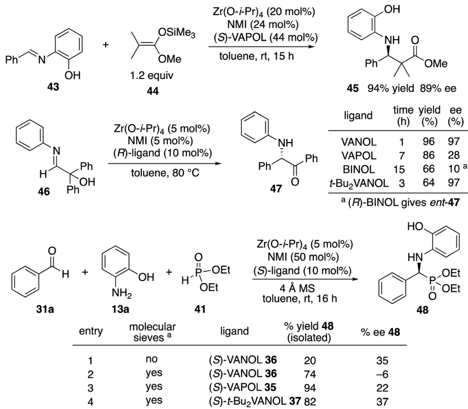
Scheme 3 Initial success with zirconium catalysts.
