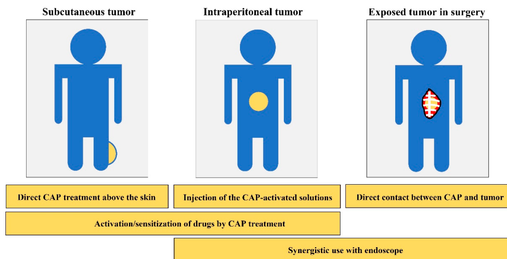
Figure 5. Schematic illustration of possible means to use CAP in clinical cancer therapy.
