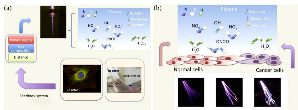
Figure 6. A schematic illustration of an adaptive plasma system. (a) Basic concept. A CAP treatment can trigger different responses in cancer cells and normal cells. An adaptive plasma system can collect, measure, record, and analyze these responses as signals. These signals provide a feedback signal to the system, which in turn modulates the chemical composition of CAP by controlling gas composition, power supply, the gap between the source and target, etc. (b) The target affects the discharge pattern of plasma by self-organization. For example, cancer cells and normal cells exhibit large differences in membrane potential, which can be used as a feedback signal to control plasma through the self-organization of plasma with different patterns and modes. The plasma adaptive therapeutic system through real-time cellular and tissue response can lead to optimal and selective cancer treatment ((a,b) are reproduced with permission from Keidar, Michael, et al. Trends in Biotechnology 36.6, 586–593, (2018). Copyright 2017 Elsevier Publisher. [107]).
