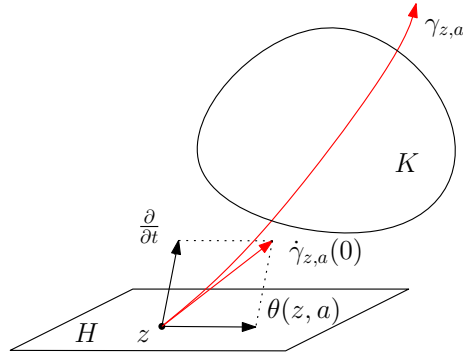
Fig. 2. Parameterization of lightlike geodesics near \gamma_0
