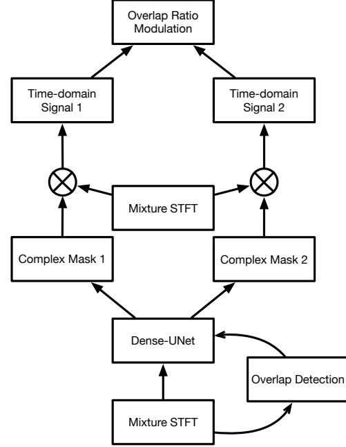
Fig. 1: Diagram of the separation model with FiLM layers. We use TCN for frame-level overlap detection.
