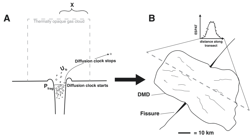
Figure 4. Schematic rendering of the eruption-diffusion model. (a) Schematic of critical stages of eruption model and (b) schematic of resulting numerical ESPAT that results from the simulated eruption. ESPAT, Effective Single Particle Absorption Thickness.
