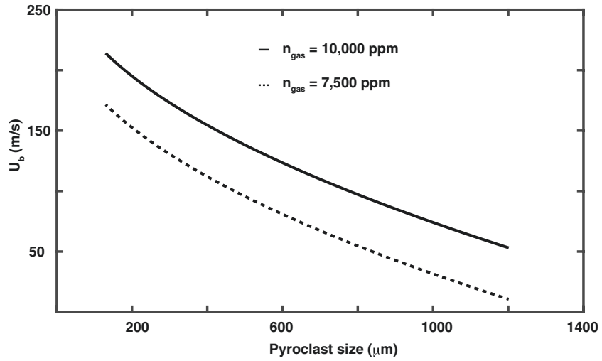
Figure 2. Schematic Initial ballistic velocities for pyroclasts, U_b , as a function of pyroclast size in diameter. The contours illustrate the dependence of U_b as a function of the concentration of exsolved volatiles upon fragmentation, n_{\text{gas}} .
