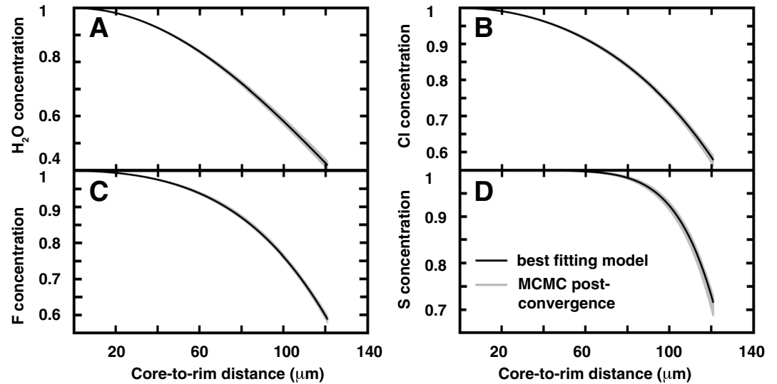
Figure 3. Diffusion plots with the normalized concentration of (a) H 2 O, (b) chlorine, (c) fluorine, and (d) sulfur. As a function of core-to-rim distance within Delano's green glass bead #5 (very low-Ti). Bold black lines represent the best solution upon convergence of MCMC. Shaded gray areas represent the model output after convergence for a given MCMC run. MCMC, Markov-Chain Monte-Carlo.
