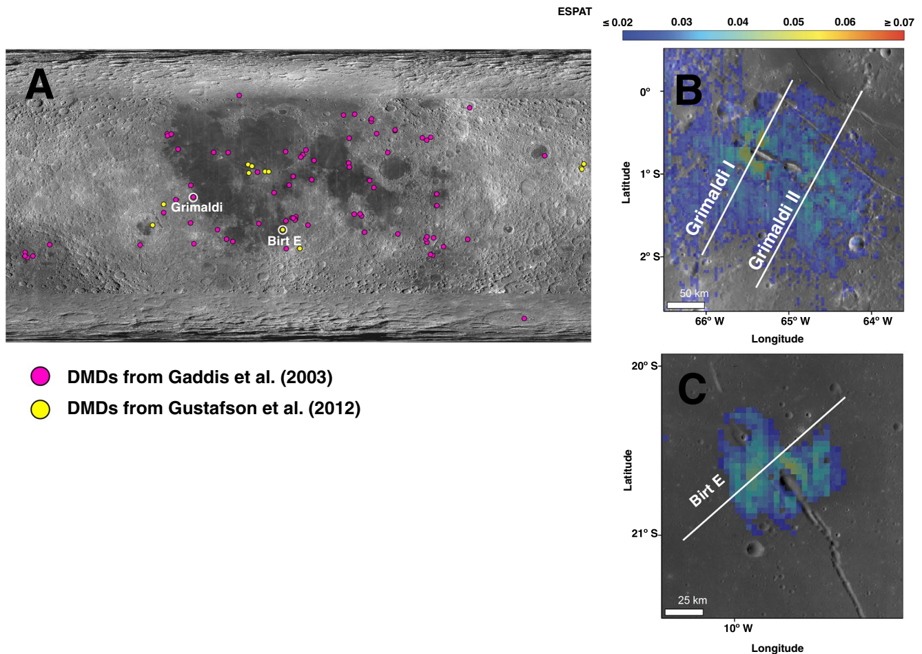
Figure 1. (a) Map of Dark-Mantle-Deposits (DMDs) in and around Procellarum Creep Terrain identified from Gustafson et al. (2012) and Gaddis et al. (2003). DMDs Grimaldi and Birt E (investigated in this study) are circled in white. (b and c) ESPAT maps and approximate transect lines of DMDs Grimaldi and Birt E, respectively. ESPAT, Effective Single Particle Absorption Thickness.
