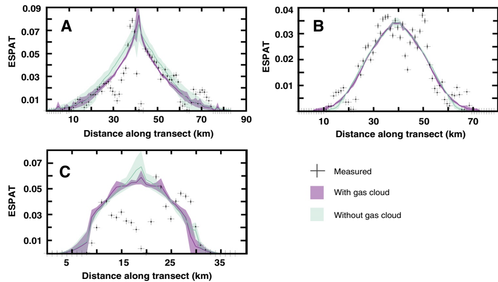
Figure 7. Best fitting models to the measured ESPAT profile for each combination of evaporation rate and cooling rate for (a) Grimaldi I, (b) Grimaldi II, and (c) Birt E. The solid line indicates the most likely solution, light shades indicate total range spanned by the posteriori distribution of the MCMC for inversions that include and neglect the presence of an opaque gas cloud. MCMC, Markov-Chain Monte-Carlo; ESPAT, Effective Single Particle Absorption Thickness.
