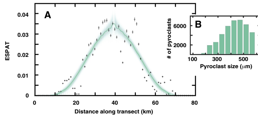
Figure 5. (a) The solid line represents the best fitting model for the second transect for the DMD Grimaldi II for an MCMC run of 10,000 iterations and an evaporation rate of 1.4 \times 10^{-6} m/s and a cooling rate of 6.4^\circ\text{C/s} . The green shaded area brackets the resulting ESPAT profiles sampled after the burn-in period ( \sim 1,000 iterations). (b) The resulting pyroclast size distribution for the best fitting model. DMD, Dark-Mantle-Deposit; MCMC, Markov-Chain Monte-Carlo; ESPAT, Effective Single Particle Absorption Thickness.
