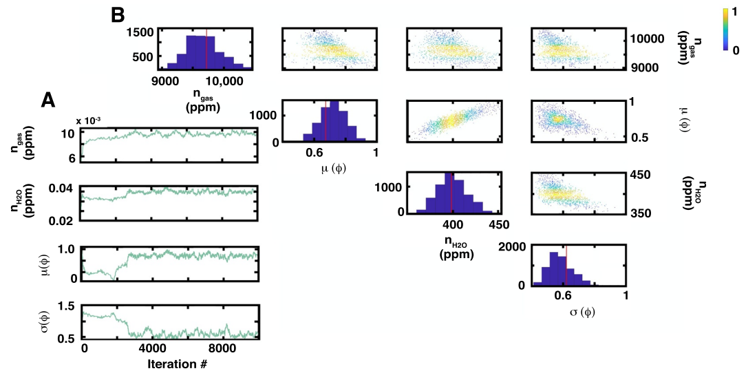
Figure 6. (a) Trace plots for MCMC run on Grimaldi II with an evaporation rate of 1.4 \times 10^{-6} m/s and a cooling rate of 6.4^\circ\text{C/s} . (b) Along diagonal of matrix of plots is the marginal posteriori distribution for each parameter with the solid red line representing the most likely solution in the parameter space, while the off-diagonal scatter plots highlight the covariance between parameters sampled from the posteriori distribution after burn-in. MCMC, Markov-Chain Monte-Carlo.
