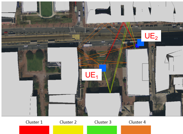
Fig. 4. NLOS scenario clustered paths, color-coded by cluster.
