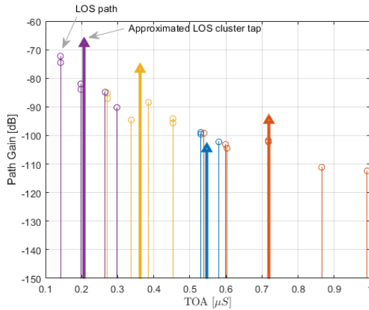
Fig. 8. LOS scenario clustered CIR and approximated CIR.
