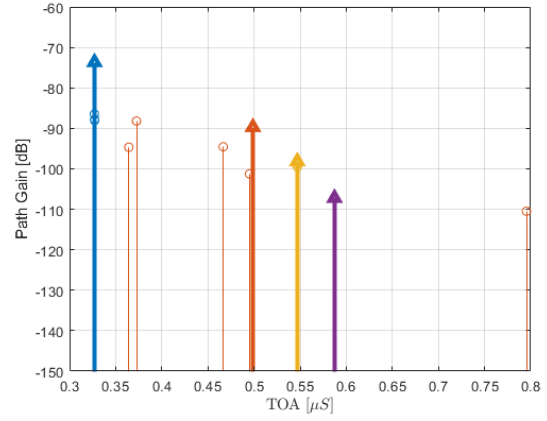
Fig. 5. NLOS scenario clustered CIR and approximated CIR.
