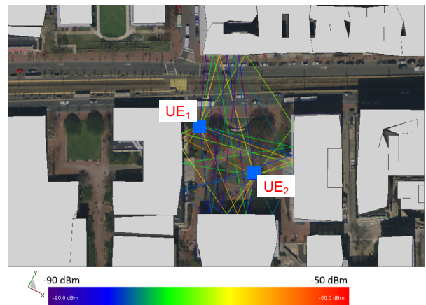
Fig. 7. LOS scenario propagation paths, color-coded by received power.
