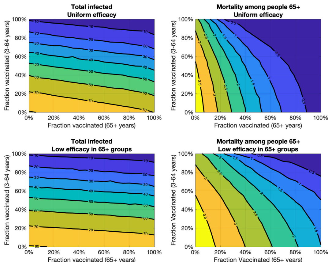
Fig. 2. Infections and mortality under different (sterilizing) vaccine uptake rates. Contour plots indicate (a,c) total percentage of the population that becomes infected and (b, d) estimated mortality among people aged \geq 65 years old. Two scenarios are shown: (a,b) constant vaccine efficacy of 90% across the whole population aged 3 and above; (c,d) vaccine efficacy of 90% among people aged 3–64 and 20% among people aged \geq 65 years.
