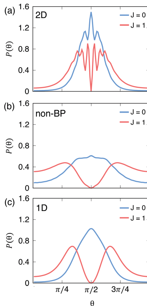
Fig. 8 The normalized photofragment angular distribution for the rovibrational wavefunction J = 0 and J = 1 . (a) 2D model. (b) non-BP model. (c) 1D model.
