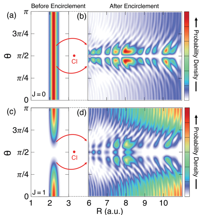
Fig. 3 The nuclear probability density obtained from the 2D model with the initial excitation to the lower polariton state |-,0\rangle . Left: Before the encirclement ( t = 0 fs) and right: after the encirclement ( t = 134 fs) for the initial rotational quantum number J = 0 (a and b) and J = 1 (c and d).
