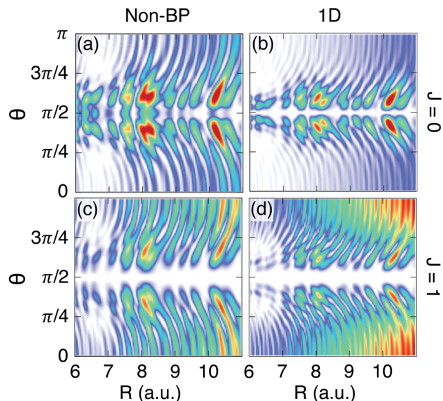
Fig. 4 The nuclear probability density of the |-,0\rangle state obtained from the non-BP and 1D models at t = 134 for the rovibrational wavefunction J = 0 (a and b) and J = 1 (c and d).
