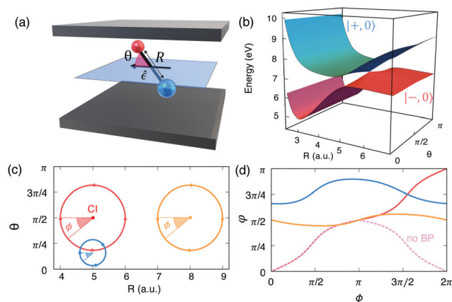
Fig. 1 (a) The angle between the polarization direction of the cavity photon mode and the direction of the molecular dipole moment. (b) The polaritonic potential energy surface ( |-,0\rangle and |+,> ) as a function of the dissociation coordinate ( R ) and the angular coordinate ( \theta ) for a cavity coupling \lambda = 0.04\sqrt{2/\hbar\omega_c} ( \kappa = 0.04 a.u.). (c) The contours used in the Berry phase calculations. (d) The transformation angle \phi (eqn (18)) as a function of the encirclement angle \phi .
