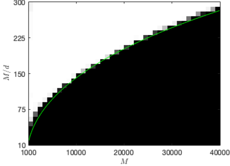
Figure 1: Empirical phase transition in the noiseless case with rank-1 measurements. The success rate out of 100 trials is plotted in a gray scale (white: all success, black: all failure).
