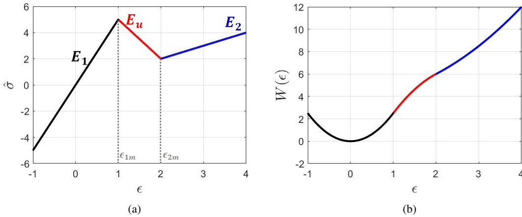
Figure 2. Material response. (a) Stress-strain curve with E_1 = 5 and E_2 = 1 . (b) Strain energy density.
