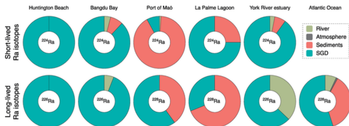
Fig. 8. Relative contribution of different sources (river, atmosphere, sediments and SGD) to the total ^{224}\text{Ra} (upper row) and long-lived Ra isotopes (lower row) for six study sites with distinct characteristics: Huntington Beach, USA (sandy intertidal beach face; Boehm et al., 2004 and Boehm et al., 2006); Bangdu Bay, Korea (semi-enclosed bay on a volcanic island; Hwang et al., 2005); Port of Maó, Spain (semi-enclosed harbor with large resuspension of sediments; Rodellas et al., 2015a, 2015b); La Palme Lagoon, France (micro-tidal coastal lagoon with karst springs; Tamborski et al., 2018); York River estuary, USA (micro-tidal estuary; Luek and Beck, 2014); Atlantic Ocean (upper 1000 m of water column; Moore et al., 2008). The sites are organized according to increasing water residence times of the study area (left to right). The Ra isotope used is indicated in the middle of the pie chart.
