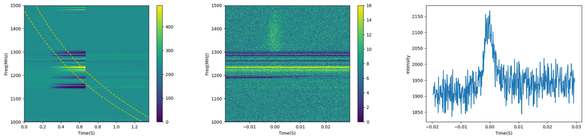
Extended Data Fig. 2. Example of a dynamic spectrum of burst with RFI.
