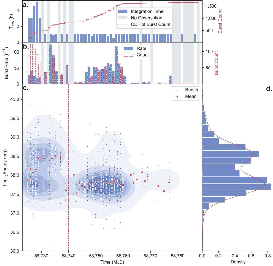
Figure 1: The detected bursts and the temporal energy distribution during the observing campaign. Panel a: the duration of each observing session (blue bar) and the cumulative number distribution of the bursts (red solid line). Panel b: the rate (blue bar) and count (red dashed line) of the bursts detected. The gray shaded bars denote days without observations. Panel c: Time dependent burst energy distribution. The blue dots are all the 1652 bursts, the red dots represent the average value for each observing session. The blue contour is the 2D Kernel Density Estimation (KDE) of the bursts. Panel d: the isotropic energy histogram of the bursts detected before MJD 58740 (14th Sept. 2019); the red dashed line represents the KDE of this distribution.
