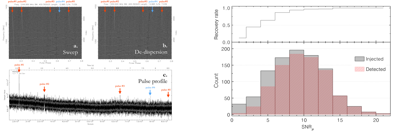
Extended Data Fig. 3. Left panel: Example of FRB simulations. Upper panels (a and b) are injected and de-dispersed dynamic spectra respectively. The time series is shown in panel (c) with the red arrows pointing to simulated pulses that were detected, while the blue arrow indicates an undetected pulse. Right panel: Comparison of \text{SNR}_p recovered by FRB search versus the corresponding injected values. The \text{SNR}_p histograms separately indicate the injected FRB pulses (grey lines) and the mock FRBs detected (red lines).
