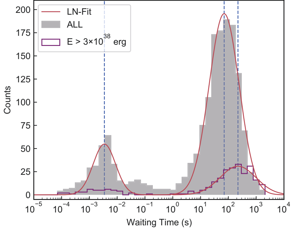
Figure 3: The waiting time distribution of the bursts. The grey bar and solid red curve denote the distribution of waiting time and its log-normal (LN) fit. The high energy component ( E > 3 \times 10^{38} erg) is shown as the solid purple line. The three fitted peak waiting times (blue dashed vertical lines) from left to right are 3.4 \pm 1.0 ms, 70 \pm 12 s, and 220 \pm 100 s, respectively. The peaks around 70 s and 220 s in the waiting time distribution are close to the average values for the respective samples (full and high energy). This is consistent with a stochastic process (see main text and Method for further discussion).
