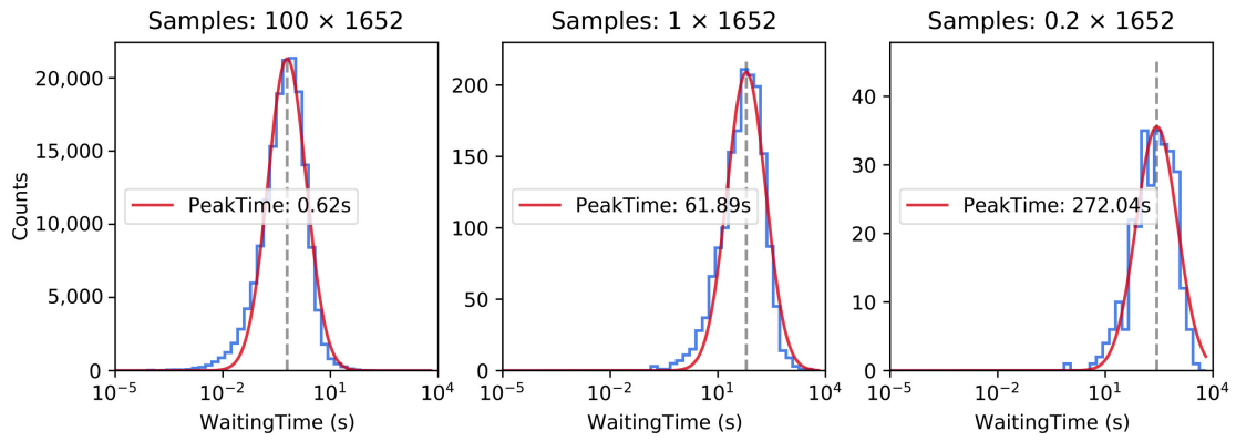
Extended Data Fig. 7. MC simulations of the waiting time distribution. The three figures correspond to three different simulations, and the number of randomly generated pulses in each simulation are 100 \times 1652 \sim 1.6e5 , 1 \times 1652 = 1652 , and 0.2 \times 1652 \sim 330 . The peak times of the three log-normal distributions are 0.62 s, 61.89 s, and 272.04 s, respectively.
