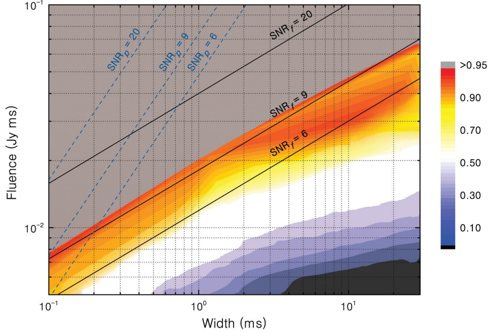
Extended Data Fig. 4. The completeness fraction of the FAST survey to FRBs as a function of the observed fluence and detected width. All FRBs lying in the integrated \text{SNR}_f < 6 region are below PRESTO's search threshold. The region above the integrated \text{SNR}_f of 6 shows the incompleteness of our FAST detection to broad FRBs as revealed by the injections. The map was smoothed (rebin) the map with a box of 0.05\text{ms} \times 0.002\text{ Jy ms} , which ensured the presence of at least one injected pulse in most map areas. Then for a few grid points without pulses, a simple linear interpolation was used to improve the visual appearance. The colour bar on the right side indicates the detection recovery fraction.
