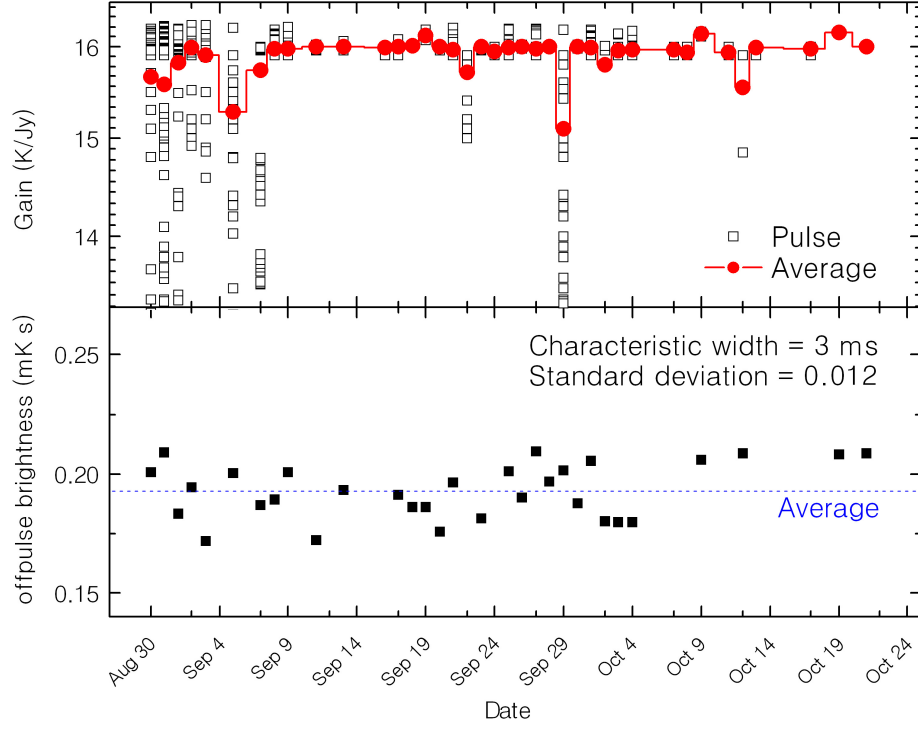
Extended Data Fig. 1. The distribution of the instrumental gain and off-pulse brightness RMS at 1.25 GHz for observations. The upper panel indicates the gain applied for each pulses. The red dots denote the averaged gain in each day. The bottom panel shows the off-pulse brightness RMS (mK s) of the first pulse detected each day.
