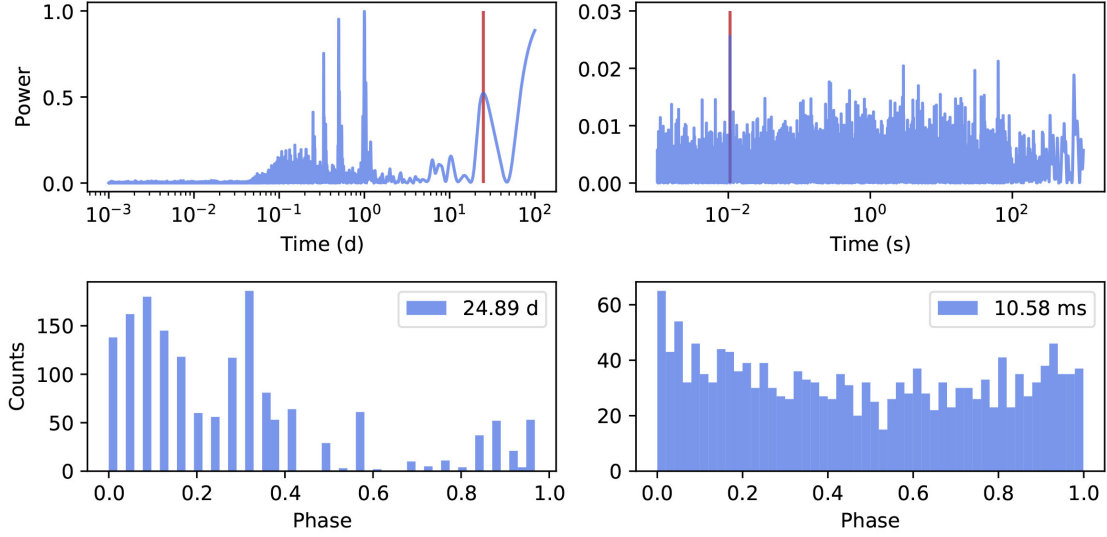
Extended Data Fig. 8. Lomb-Scargle periodograms of FRB 121102 burst arrival times (top row) along with phase histograms for two trial periods (bottom row). Left: Periods from 10^{-3} to 10^2 d. The four leftmost peaks in the periodogram are caused by daily sampling and its harmonics. The peak at \sim 24 d is related to the sampling window function (i.e. non-uniform sampling) over the 47 d data set, as is consistent with the broad distribution in burst phase (bottom left). Right: Periods from 1 ms to 10^3 s. The peak at 10 ms is a large multiple of the original sampling time and also yields no distinct concentration in burst phase.
