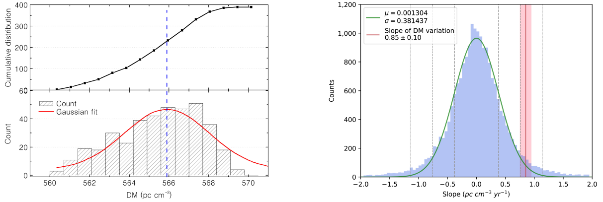
Extended Data Fig. 10. Left panel: Histogram and cumulative distribution of dispersion measure for FRB 121102. Right panel: Slope distribution of null hypothesis test.
