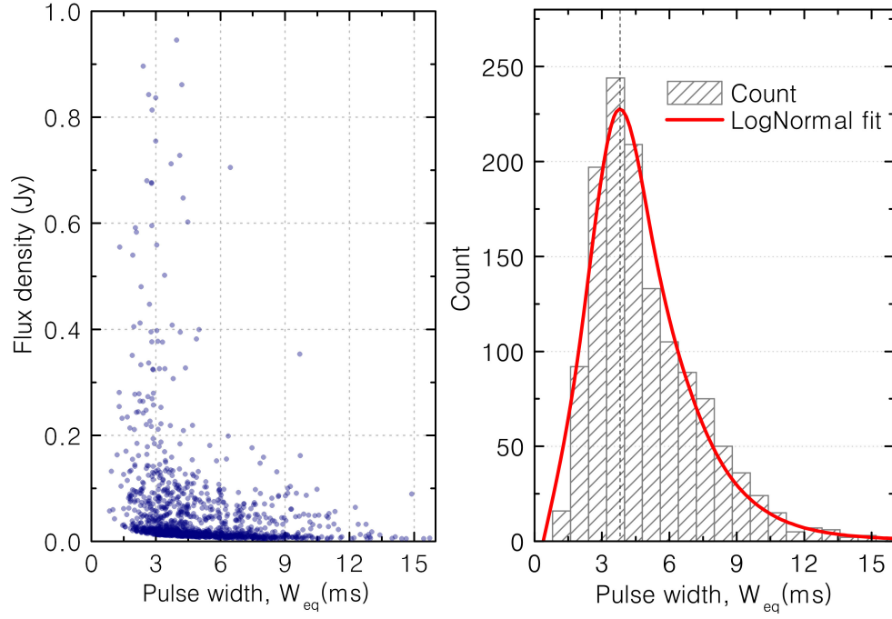
Extended Data Fig. 6. Flux intensity and pulse width distribution of FRB 121102. Left: Flux intensity against pulse width for the FRB 121102 bursts with peak \text{SNR}_p > 10 in our sample. Right: The equivalent pulse width histogram.
