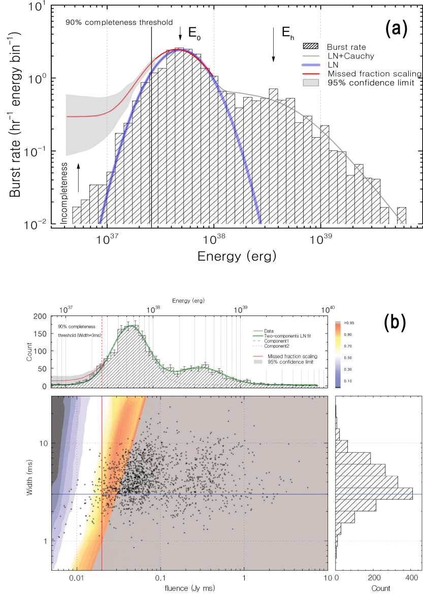
Extended Data Fig. 5. Upper panel (a): The burst rate distribution of the isotropic equivalent energy. Details as per Extended Data Fig. 2. The red line represents the recovered distribution by adding back the missing fraction based on the simulation. The grey shaded region is the uncertainty for a 95% confidence based on the Poisson statistical assumption in the "reconstructed" fitting. Bottom panel (b): The fluence-width distribution at 1.25 GHz for FRB 121102 bursts. The black dots indicate the 1,652 detected bursts, the colorbar is consistent with Extended Data Fig. 4. In the upper panel, the two-component lognormal (LN) distribution is separately fitted in blue dashed line and grey dot line, an overall fit for bursts is shown in green. The red line and the shaded region indicates reconstructed missing fraction of bursts detection and uncertainty.
