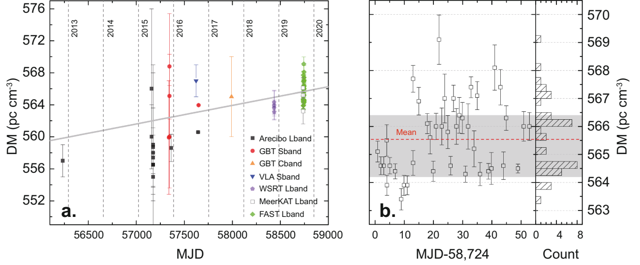
Figure 4: The DM evolution of FRB 121102. Left panel (a): Temporal DM variation for FRB 121102 over a nine-year period. The solid grey line denotes the linear fit with slope +0.85 \pm 0.10 pc cm -3 yr -1 . Right panel (b): the distribution of DM estimates for the brightest burst on each day of FAST observations. The red dashed line indicates the average DM of 565.6 pc cm -3 during the FAST observations, and the grey region shows the 95% confidence level.
