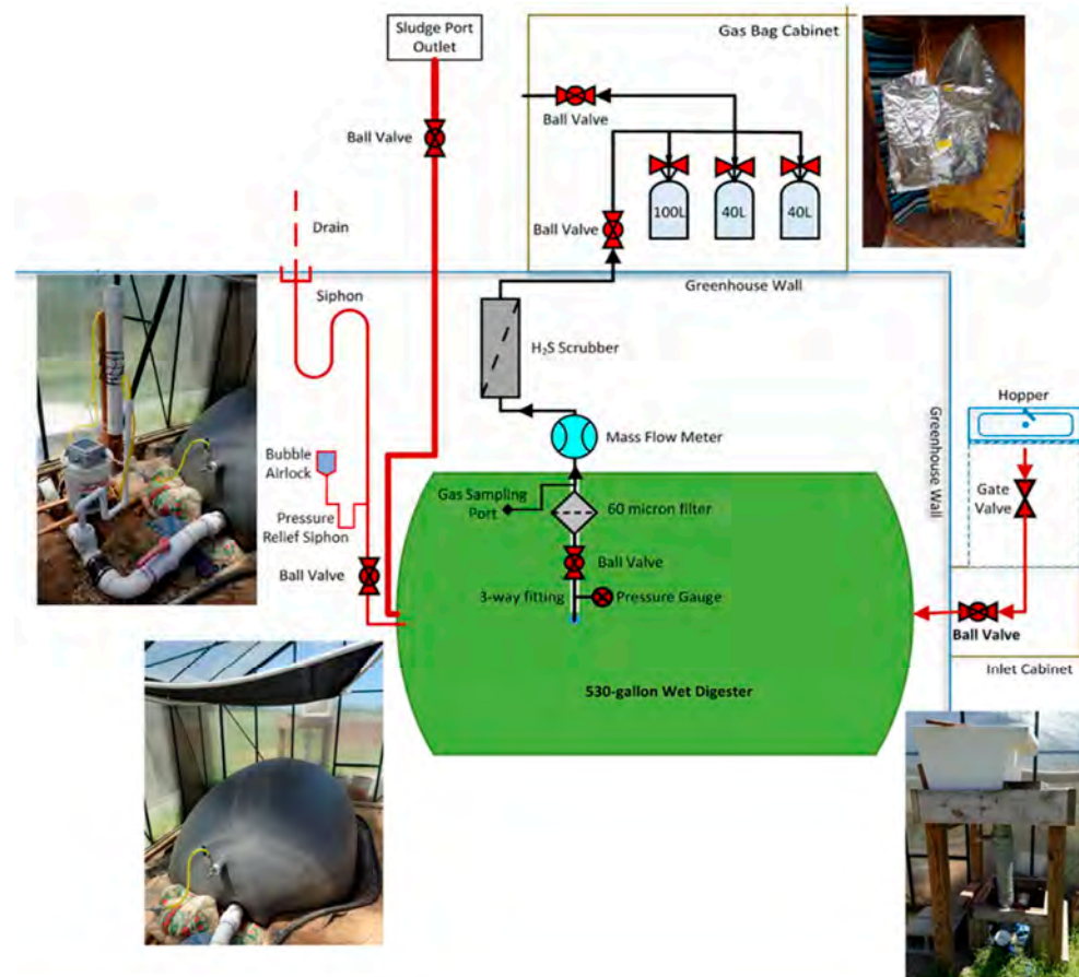
Figure 1. Schematic of the digester and greenhouse setup, modified from Miller et al. 2020 [22]. Black lines indicate stainless steel or Tygon fuel line tubing and fixtures; red lines indicate PVC fittings and tubing.
