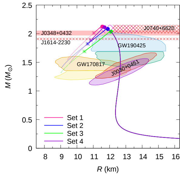
Figure 6. (Color online) M – R relationship of the selected EoSs (Table 4) of this work. The solid dots indicate the appearance of color superconducting quark matter in HSs, which happens just before the maximum-mass peaks are reached. For a rapid conversion of matter, the stellar configurations to the left of each maximum-mass star are unstable. For slow conversions there exist extended branches of stable stars which end at the locations marked with asterisks. The shaded regions (clouds) correspond to constraints imposed by GW170817, GW190425, and NICER observations of PSR J0030+0451. The horizontal pink striped bands, indicate constraints imposed by pulsars J0740+6620, J0348+0432, and J1614-2230.
