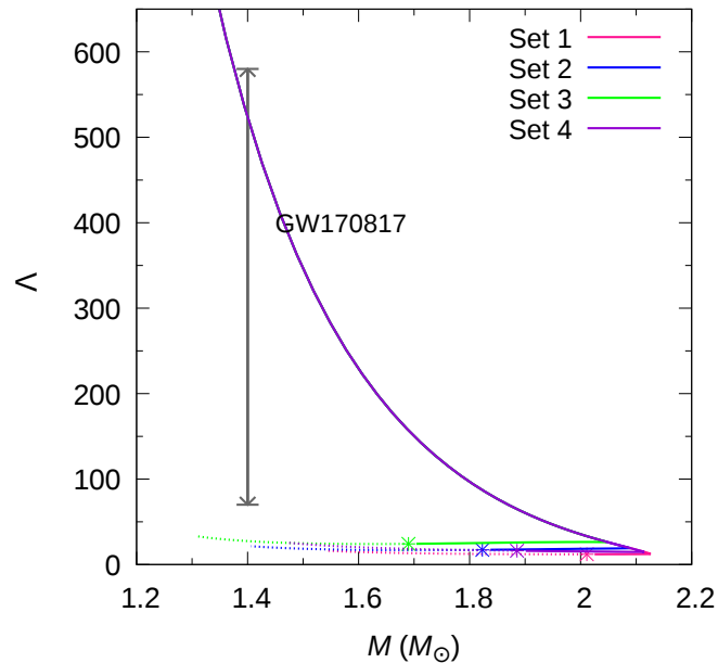
Figure 7. (Color online) Dimensionless tidal deformability as a function of gravitational mass, with the constraint obtained from GW170817 [5]. Stable stellar configurations beyond the maximum mass have very small values of \Lambda , which are almost independent of mass. The positions of the terminal stars of the twin HSs branch (obtained for slow hadron-quark conversion) are marked with asterisks.
