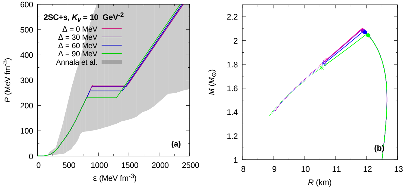
Figure 3. Hybrid EoS (panel (a)) and mass-radius relationship (panel (b)) for the 2SC+s phase at fixed gap value of K_V = 10 \text{ GeV}^{-2} , for different values of the \Delta parameter. In panel (a), the grey region shows the constraints presented in [42]. The solid dots in panel (b) indicate the appearance of the color superconducting phase, just before the maximum mass peak. For rapid conversions, the stellar configurations to the left of each maximum mass are unstable and the existence of HSs is only marginal. For slow conversions, an extended stability branch exists. The stable configurations are shown by continuous lines. The terminal configurations are marked with asterisks.
