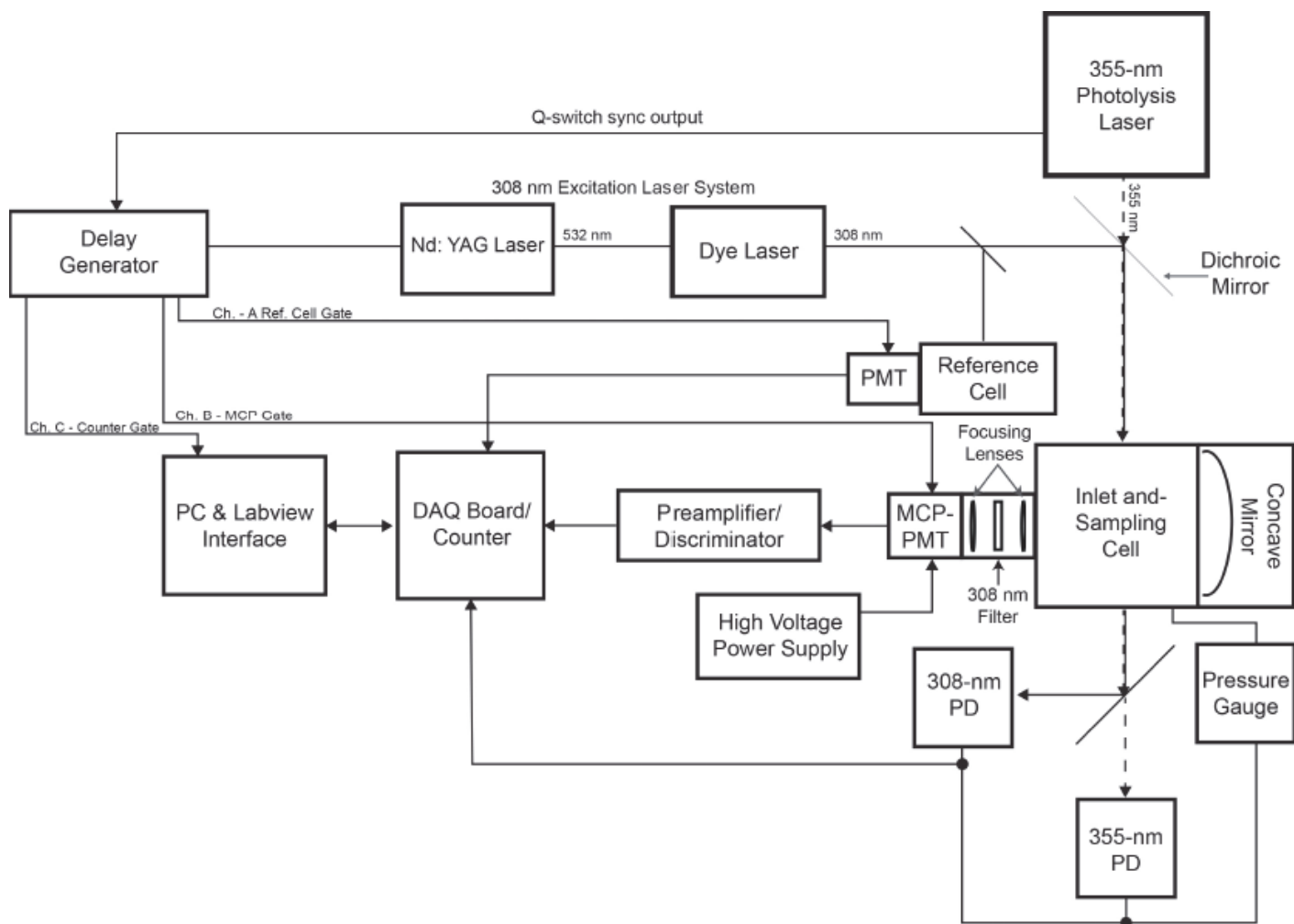
Figure 1: Schematic diagram of the LP/LIF instrument.
