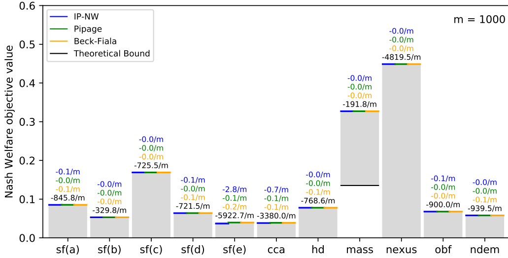
Figure 3: m = 1000 . Shaded regions extend from NW(p^*) , the fairness of the optimal unconstrained distribution, down to the minimum fairness implied by the tightest theoretical upper bound in that instance (in all instances but “obf” Theorem 3.3 is tightest). Each algorithm or bound’s loss relative to NW(p^*) is written above in the corresponding color. PIPAGE NW values are the average of 1000 runs (standard deviation < 10e-17 in all instances).
