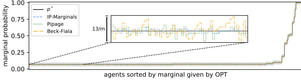
Figure 2: Instance = sf(a), m = 1000 . Line plot shows the Leximin-optimal marginals \pi^* , along with marginals given by all algorithms sorted according to \pi^* . Note that each x coordinate then corresponds to an individual. The zoomed box shows the magnitude of marginal discrepancy around \pi^* . The surrounding shaded region shows the tightest theoretical bound on the marginal discrepancy, in this case from Theorem 3.3, around the optimal marginals. PIPAGE marginals are the average of 1000 runs (max standard deviation in any marginal was < 10e-14 ).
