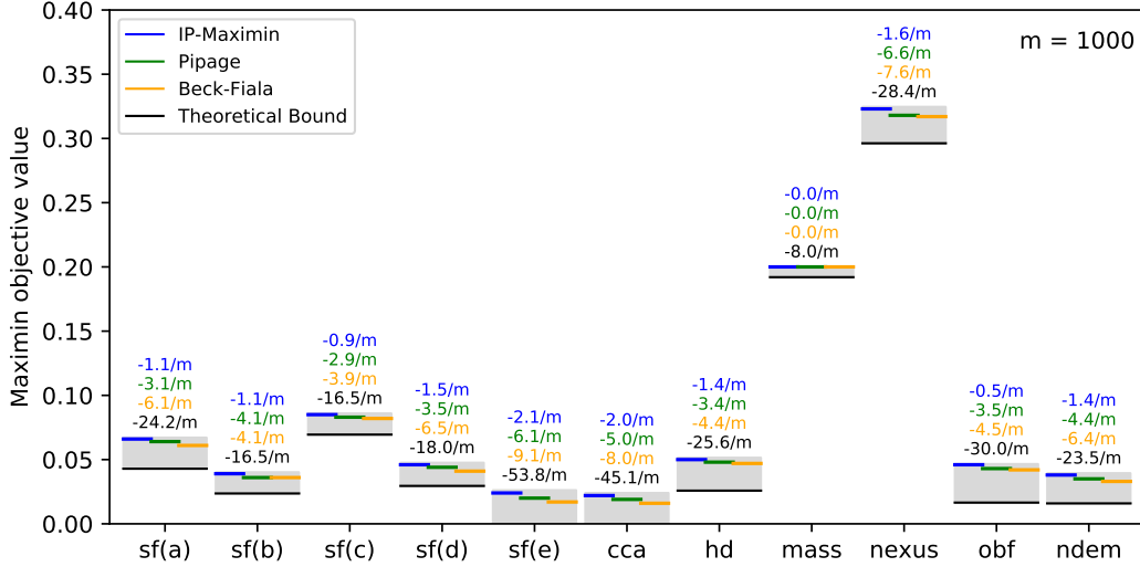
Figure 1: m = 1000 . Shaded regions extend from \text{Maximin}(p^*) , the fairness of the optimal unconstrained distribution, down to the minimum fairness implied by the tightest theoretical upper bound in that instance (in all instances but “obf” Theorem 3.3 is tightest). Each algorithm or bound’s loss relative to \text{Maximin}(p^*) is written above in the corresponding color. PIPAGE Maximin values are the average of 1000 runs (max standard deviation across instances was < 10e-17 ).
