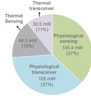
Fig. 15. Power distribution of FaceSense
