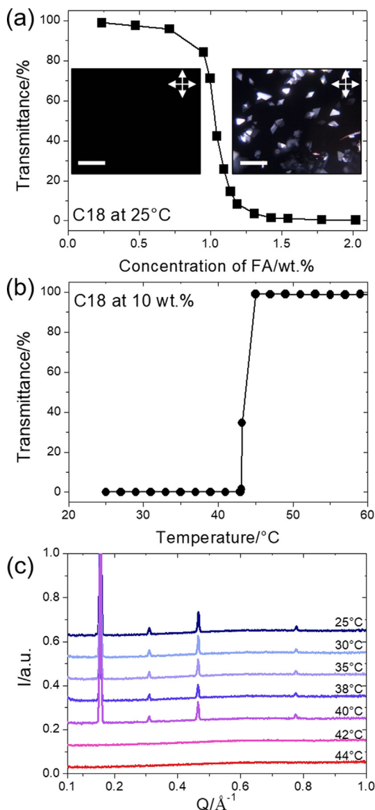
Fig. 2. (a) Evolution of the transmittance as a function of fatty acid concentration in 85% of ethanol with 15% water (v/v) at 25 °C. The cross-polarized light microscopy pictures show the absence of crystals below 1 wt% and the presence of crystals (bright spots) at 10 wt%. The scale bars are 100 \mu\text{m} . (b) Evolution of the transmittance as a function of temperature for C18 at 10 wt% in 85% of ethanol. (c) WAXS spectra for C18 at 10 wt% in 85% of ethanol as a function of temperature. The spectra are shifted in intensity for clarity.
