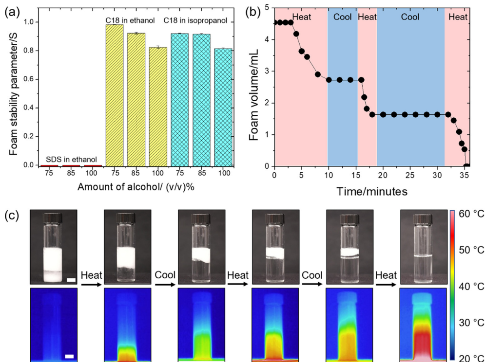
Fig. 4. (a) Evolution of the foam stability parameter ( S ) for C18 at 10 wt% and SDS at 10 wt% with an amount of alcohol varying from 75% to 100% at 25 °C. Stabilization/destabilization of a foam made with C18 at 10 wt% in 85% of ethanol during heating/cooling cycles: (b) Evolution of the foam volume as a function of time. (c) Photographs of foams with the corresponding Infrared images. The scale bar is 5 mm.
