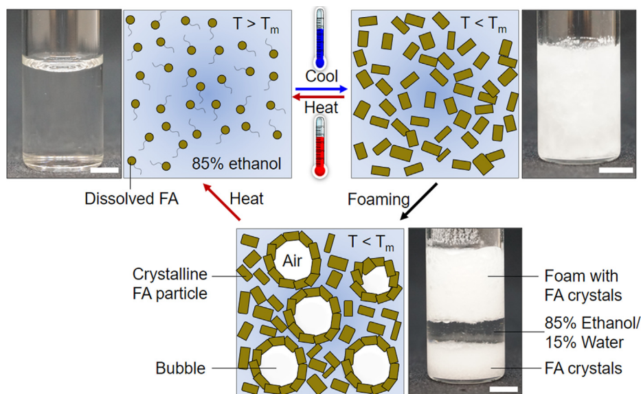
Fig. 1. Schematic of the transparent sample containing molecularly dissolved fatty acids (FA) in the solvent at temperature above the melting temperature ( T_m ). Below T_m , crystals are formed by cooling, and a turbid dispersion is obtained. By introducing air into the dispersion, foams are formed due to the bubbles being stabilized by the FA crystals. By heating the foam above T_m , the crystals melt, and the foam disappears leading to the initial transparent solution of FA molecules. The scale bar is 5 mm.
