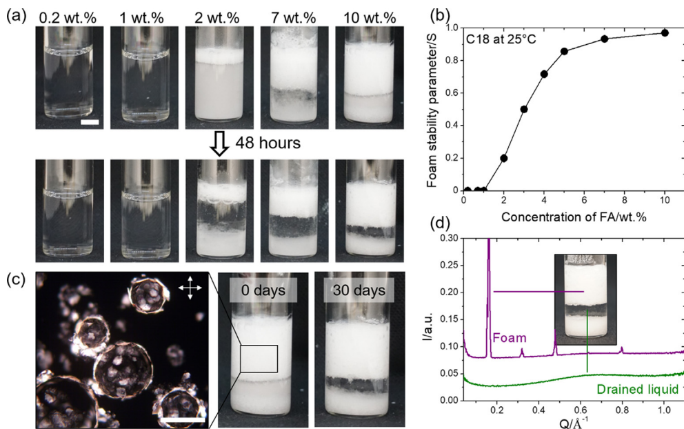
Fig. 3. (a) Photographs of the change in foam volume as a function of C18 concentration just after the foam formation and after 48 h at rest at 25 °C. The scale bar is 5 mm. (b) Change in the foam stability quantified using the foam stability parameter ( S ) as a function of C18 concentration at 25 °C. (c) Photographs of a foam made with C18 at 10 wt% just after foam formation and after conservation of the foam for 30 days at 25 °C, with the corresponding cross polarized light microscopy image showing the bubbles coverage by fatty acid crystalline particles and the non-spherical shape of the air bubbles. The scale bar is 50 \mu\text{m} . (d) WAXS spectra of the foam and the drained transparent liquid at 25 °C.
