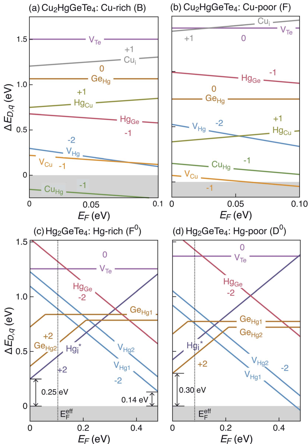
Fig. 4 Defect formation energy for native point defects as a function of Fermi energy ( E_F ) in \text{Cu}_2\text{HgGeTe}_4 under (a) Cu-rich and (b) Cu-poor conditions. Cu interstitials \text{Cu}_i are placed in the tetrahedral interstitial site. Defect formation energy for native point defects as a function of Fermi energy in \text{Hg}_2\text{GeTe}_4 under (c) Hg-rich and (d) Hg-poor conditions. Interstitials \text{H}_i^* are placed in the vacant site of the ordered vacancy compound. The effective Fermi energy is shown by the dashed vertical line, which is the position of Fermi energy when the system is quenched from the synthesis temperature. For \text{Hg}_2\text{GeTe}_4 , the positive energy windows \Delta E_{\text{don}} of 0.14 eV and \Delta E_{\text{acc}} of 0.25 eV are favorable for p- and n-type extrinsic doping.
