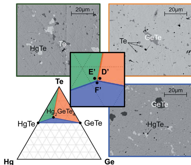
Fig. 3 Phase stability region of \text{Hg}_2\text{GeTe}_4 in composition space with SEM images of samples at different growth conditions. E^0 , D^0 , and F^0 match the same labels in Fig. 2(d).
