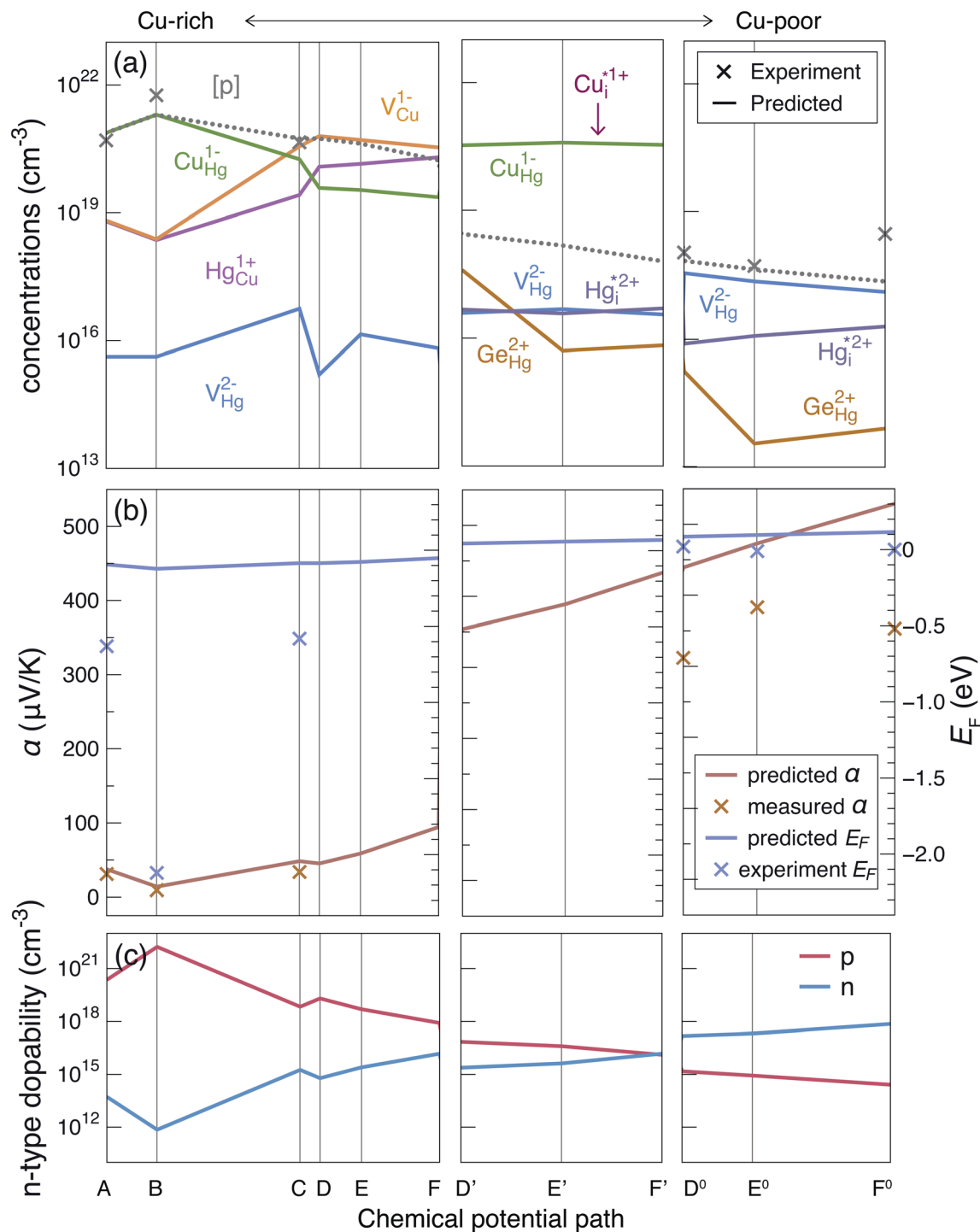
Fig. 6 Brouwer band diagram of transport properties plotted along the chemical potential path from \text{Cu}_2\text{HgGeTe}_4 to \text{Hg}_2\text{GeTe}_4 at T = 50^\circ . (a) Defect concentrations (solid lines) and carrier concentrations (dashed lines) from first-principles defect calculations and experiment Hall measurements (x symbols). (b) Seebeck coefficient ( \alpha ) shown together with position of Fermi energy ( E_F ) reference to VBM for that material. (c) Ideal n-type dopability represented by maximum achievable electron concentrations, with labels for both electron (blue) and hole (red) concentrations.
