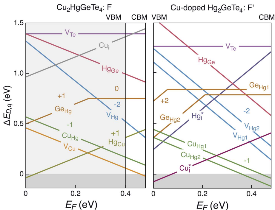
Fig. 5 Comparison of defect chemistry for Cu-doped \text{Hg}_2\text{GeTe}_4 and \text{Cu}_2\text{HgGeTe}_4 at the same set of chemical potentials. In the ternary, interstitials \text{Cu}_i^* and \text{H}_i^* are placed in the vacant site of the ordered vacancy compound. The energy domain for \text{Cu}_2\text{HgGeTe}_4 has been widened to reproduce the band gap for \text{Hg}_2\text{GeTe}_4 ( \Delta E_{\text{VBM}} = -0.38 eV). The shift of valence band is shaded in grey for \text{Cu}_2\text{HgGeTe}_4 . To facilitate comparison, defects that correspond to each other are shown in the same color for both materials.
