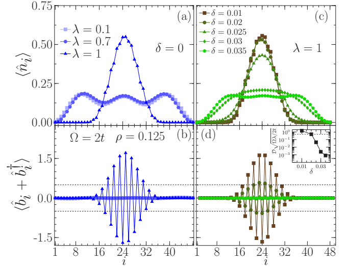
FIG. 3. GS expectation values of the average occupation number \langle \hat{n}_i \rangle [(a),(c)], lattice distortion \langle b_i + b_i^\dagger \rangle [(b),(d)]. The results were obtained for a chain with L = 48 and OBC and with N = 6 electrons ( \rho = 0.125 ) and at phonon frequency \Omega = 2t . Panels (a) and (b) show results for various \lambda for dispersionless phonons \delta = 0 . Panels (c) and (d) show results for various \delta at strong coupling \lambda = 1 corresponding to the unphysical regime. Inset of (d) shows the staggered displacement amplitude [Eq. (1)] as a function of \delta ; the horizontal red dashed line at 1/2 sets the limit of physicality for the phonon displacements.
