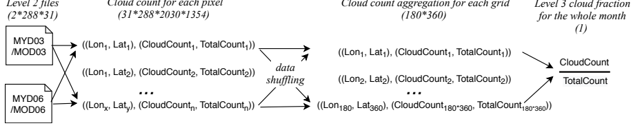
Fig. 4. Illustration of pixel level parallel aggregation.
