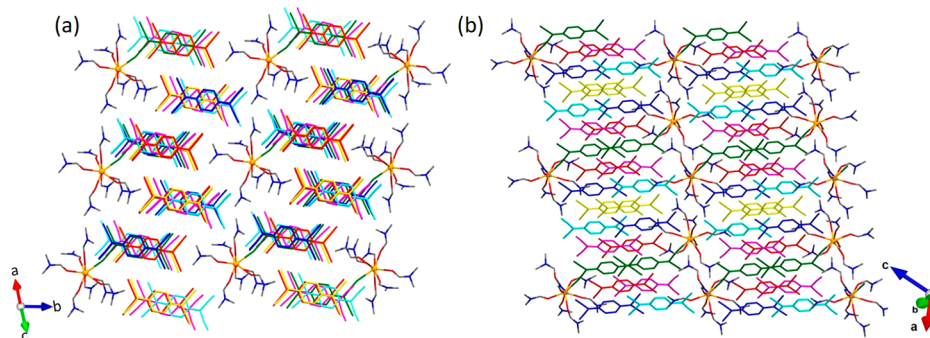
Figure 6. (a) The top view of the one-dimensional stacks of \text{TCNQ}^{\delta-} anions in the crystal packing of 3 . (b) The side view of the \pi – \pi stacking between \text{TCNQ}^{\delta-} anions. Different colors are used to label crystallographically distinct TCNQ units. The color scheme for other atoms: Nd = orange, O = red, N = blue, C = gray. Hydrogen atoms are omitted for clarity.
