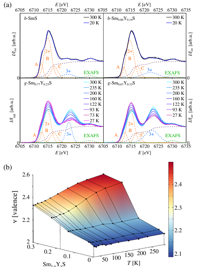
FIG. 2. (a) Temperature dependence of the Sm- L_3 PFY-XAS spectra for b\text{-SmS} , b\text{-Sm}_{0.86}\text{Y}_{0.14}\text{S} , g\text{-Sm}_{0.77}\text{Y}_{0.23}\text{S} , and g\text{-Sm}_{0.67}\text{Y}_{0.33}\text{S} , respectively. The dashed lines display the best fit to the base temperature data. (b) Temperature and doping dependence of the Sm valence.
