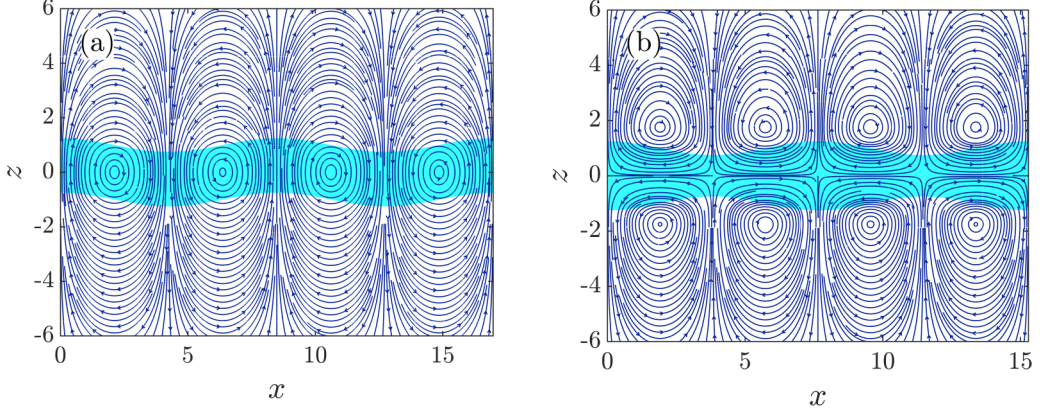
FIG. 2. Streamlines of the flow in the two dominant modes of linear instability: (a) in-phase (sinuous) mode when R = 2 and (b) antiphase (varicose) mode when R = 0.5 . Other parameters are (Q, \lambda, Ca_E, Re_E) = (1, 1, 10, 1) in both systems. The blue region illustrates a typical shape of the film in the dominant mode.
