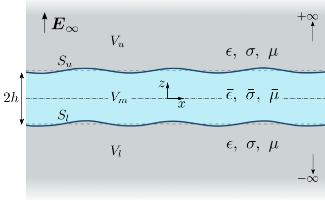
FIG. 1. Problem definition: A liquid film suspended between two semi-infinite immiscible liquid layers is subject to a perpendicular electric field E_\infty .
