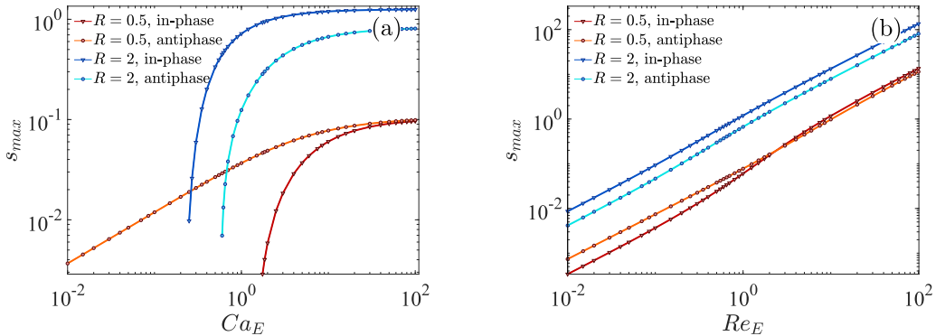
FIG. 5. Maximum growth rate in each mode of instability as a function of (a) electric capillary number and (b) electric Reynolds number for two different systems with R = 0.5 and R = 2 while (Q, \lambda) = (1, 1) . \text{Re}_E = 1 in (a) and \text{Ca}_E = 10 in (b) (identical systems studied in Fig. 4).
