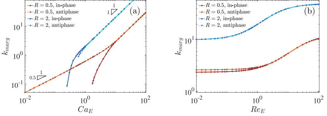
FIG. 4. Wave number k_{\text{marg}} corresponding to marginally stable perturbations ( \sigma_{\text{marg}} = 0 ) in different modes of instability as a function of (a) electric capillary number and (b) electric Reynolds number for two different systems with R = 0.5 and R = 2 while (Q, \lambda) = (1, 1) . \text{Re}_E = 1 in (a) and \text{Ca}_E = 10 in (b).
