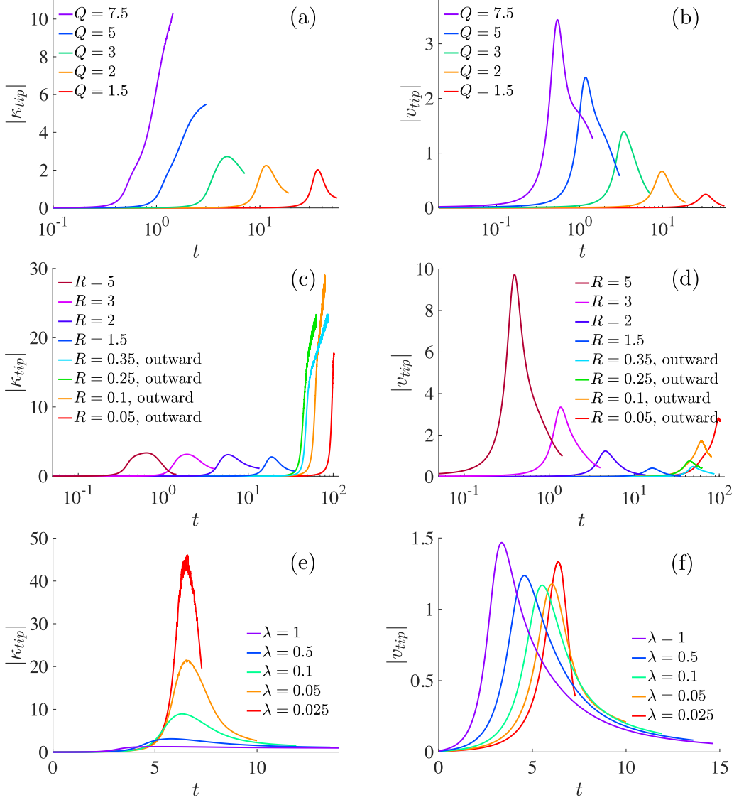
FIG. 14. Evolution of the inward and outward jets during in-phase instability as a function of (a,b) permittivity ratio in system S4, (c,d) conductivity ratio in system S6, and (e,f) viscosity ratio in system S7. Left and right columns show the evolution of the tip curvature and vertical tip velocity, respectively.
