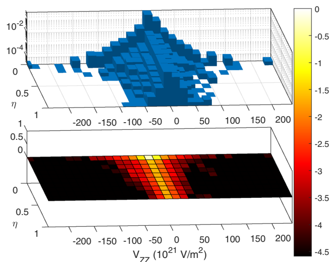
Fig. 5 Histogram (above) and intensity map (below) of the probability are shown as a function of V_{zz} and \eta . The logarithmic z-scale allows for the strong preponderance of small V_{zz} and small \eta values to be clearly seen, while at the same time revealing the bell-shaped distribution in V_{zz} for all \eta values. Values where V_{zz}=0 , and therefore \eta is ill-defined, have been excluded.
