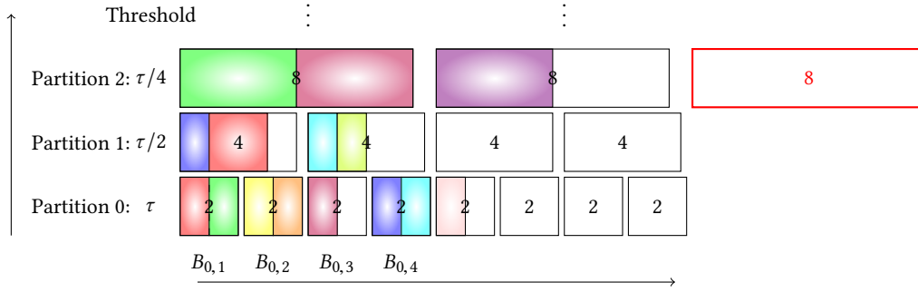
Figure 1: Partitions and buckets: B_{1,1} and B_{2,2} are partially occupied. B_{2,3} (in red) has been dynamically created, since the elements of B_{2,1} and B_{2,2} are large.
