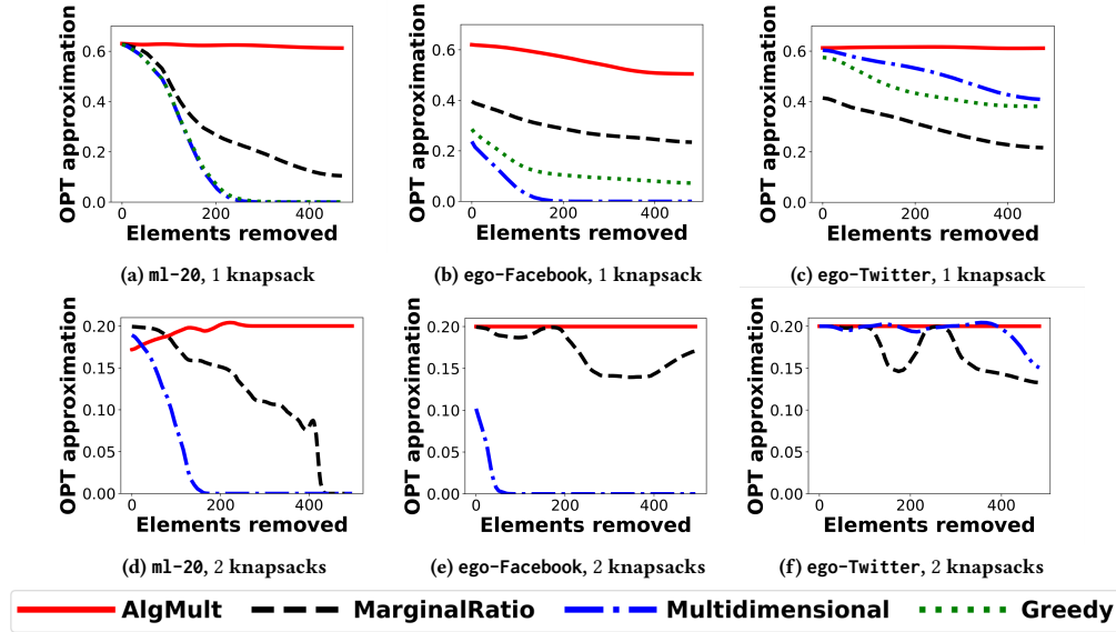
Figure 2: Approximation of f(OPT) for different algorithms ( K = 10 ). In most cases, ALGMULT outperforms the other algorithms and achieves the best possible approximation factor ( 1 - \frac{1}{e} \approx 0.63 for one knapsack, 0.2 for two knapsacks).
