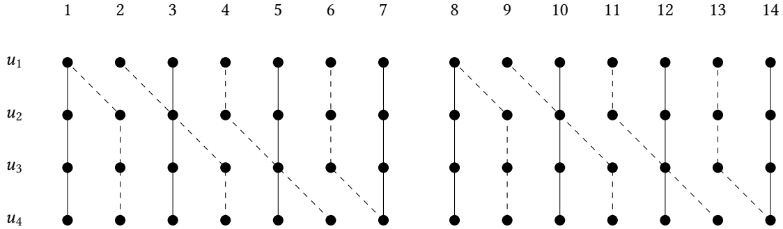
Fig. 1. A schematic diagram of the branches for an edge e = (u_1, u_2, u_3, u_4) of V label cover instance \Psi with parameters k = 4 and L = 2 . The i th row represents \pi_i^{(e)} and the j th column represents the input j . The dashed and dotted lines are to indicated the two different branches with the same values with respect to \pi^{(e)} . For example, we may deduce from this diagram that (10, 10, 10, 10) and (9, 10, 11, 11) are two branches of e . In particular, we have that \pi_1^{(e)}(9) = \pi_2^{(e)}(10) = \pi_3^{(e)}(11) = \pi_4^{(e)}(11) . Note that \psi_i^{(e)}(j) = \perp exactly when the node of the i th row and j th column is at the intersection of two branches. Compare with Figure 1 of [18].
