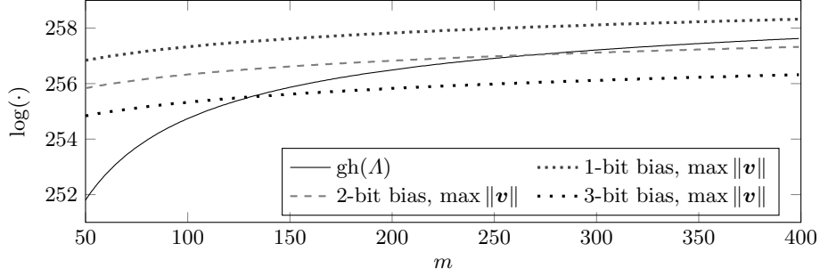
Fig. 2: Illustrating the “lattice barrier”. BDD is expected to become feasible when the length of the target vector \|\mathbf{v}\| is less than the Gaussian heuristic \text{gh}(\Lambda) ; we plot the upper bound in Equation (3) for \log(n) = 256 against varying number of samples m .
