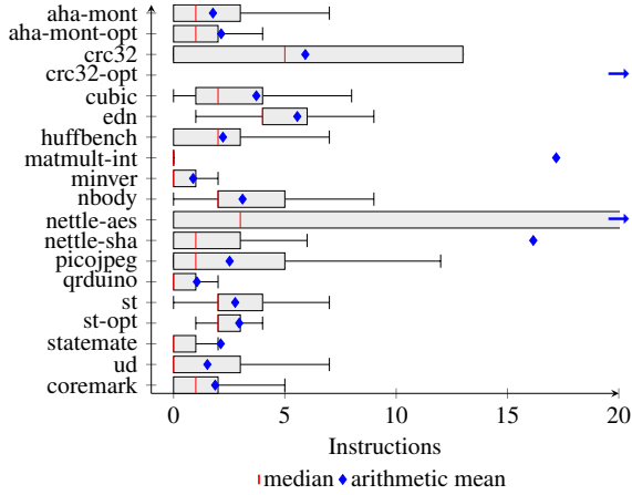
Figure 7: Distribution of instruction rescheduling per basic block, weighted by the number of invocations, dynamically derived from the hotspot analysis.
