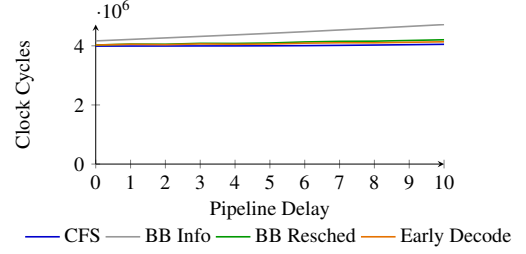
Figure 8: Influence of additional pipeline stages on the execution time for the benchmark matmult-int on VexRiscv.
