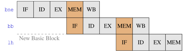
Figure 3: The worst case scenario has a branch instruction at the end of a basic block.
