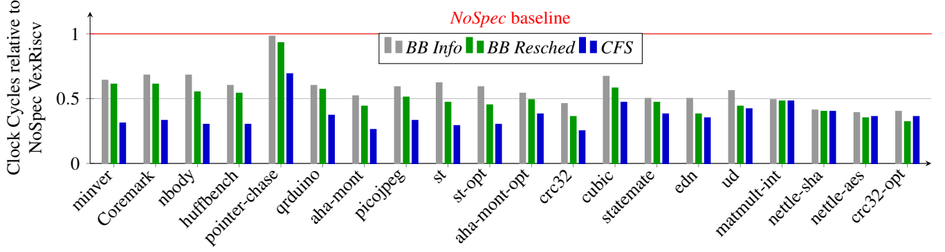
Figure 4: Performance results for various benchmarks on VexRiscv measured in clock cycles. The results are relative to the NoSpec configuration of VexRiscv (red line). Sorted descended by speedup delta in BB Resched vs CFS case. Lower delta is better. For abbreviations see Tables 1 and 2.
