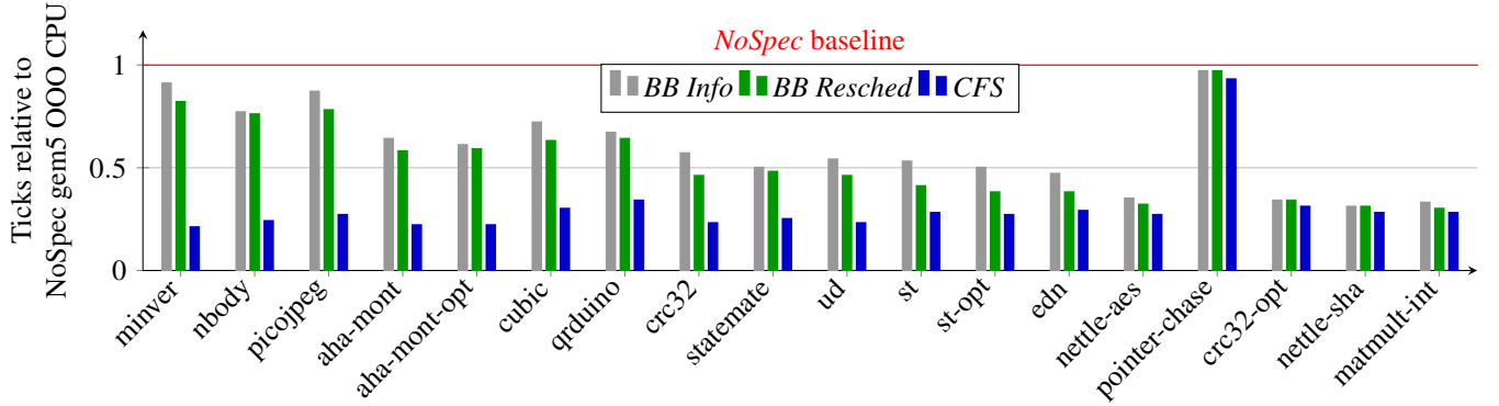
Figure 5: Performance results for various benchmarks on gem5 measured in simulation ticks. The results are relative to the NoSpec configuration of gem5 (red line). Sorted descended by speedup delta in BB Resched vs CFS case. Lower delta is better. For abbreviations see Tables 1 and 2. Huffbench and Coremark did not compile for the 64-bit target.
