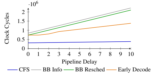
Figure 9: Influence of additional pipeline stages on the execution time for the benchmark minver on VexRiscv.
