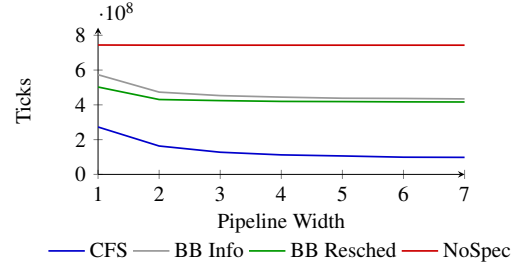
Figure 11: Influence of superscalarity on the performance of BasicBlocker using the minver benchmark on gem5.
