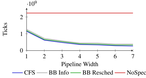
Figure 10: Influence of superscalarity on the performance of BasicBlocker using the matmult-int benchmark on gem5.
