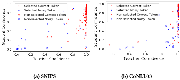
Figure 2: Visualization of MetaST re-weighting examples on SNIPS and CoNLL03 (EN).
