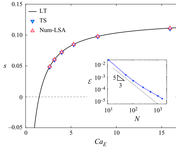
Figure 5. Growth rate s as a function of Ca_E obtained by Num-LSA, LT and TS for (R, Q, \lambda, Re_E) = (2, 3, 1, 1) . Inset shows the decay of the numerical error \epsilon with the grid size N for Ca_E = 7.96 .
