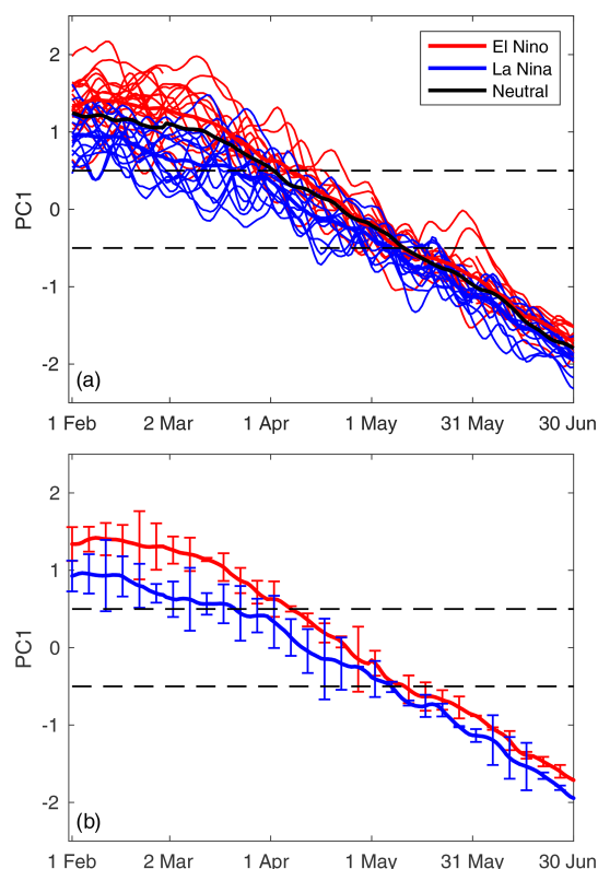
Figure 8. (a) The thin lines show PC1 values (using JRA-55) during months of La Niña events (blue) and El Niño events (red), with the thick blue (red) line showing the average La Niña (El Niño) periods. The thick black line shows the PC1 average for the remaining neutral months. Panel (b) shows the bootstrapped confidence intervals for the mean PC1 values for La Niña events (blue) and El Niño events (red).
