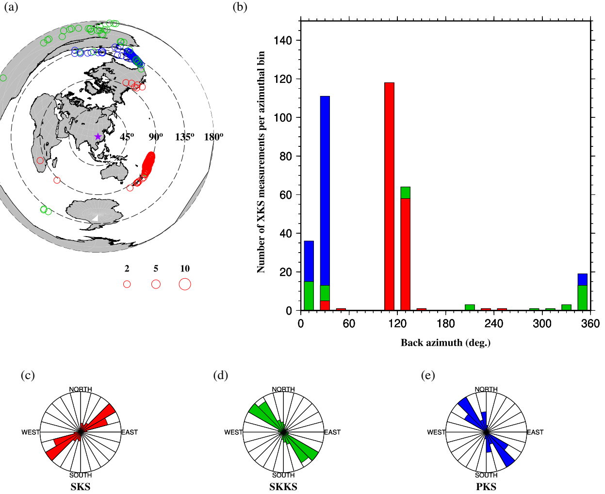
Figure 2. Events location. (a) An azimuthal equidistant projection map showing the spatial distribution of the earthquakes (circles) centred at the study area (purple star). The radius of the circles is proportional to the number of quality A or B SWS measurements from the events. (b) A histogram of the backazimuthal distribution measured by the SWS measurements. (c–e) Rose diagrams illustrating the fast orientations of the SKS, SKKS and PKS phases. For all the plots, red, green and blue colours represent the SKS, SKKS and PKS events or measurements.
