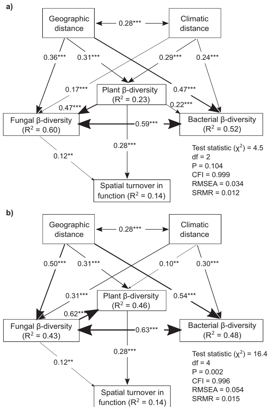
Fig. 3. Effects of geographic distance, climatic distance, and \beta -diversity on spatial turnover in ecosystem function. Plant \beta -diversity affects soil microbial \beta -diversity (a) and vice versa (b). Numbers next to arrows represent standardized path coefficients ( \beta_{std} ). Double-headed arrows represent residual correlations. Width of the arrows is scaled to the magnitude of \beta_{std} . R^2 represents the proportion of variance explained by the predictors. Indices of goodness-of-fit are given including \chi^2 statistic, degree of freedom, P value of the test statistic, comparative fit index (CFI), root mean square error of approximation (RMSEA), and standardized root mean square residual
