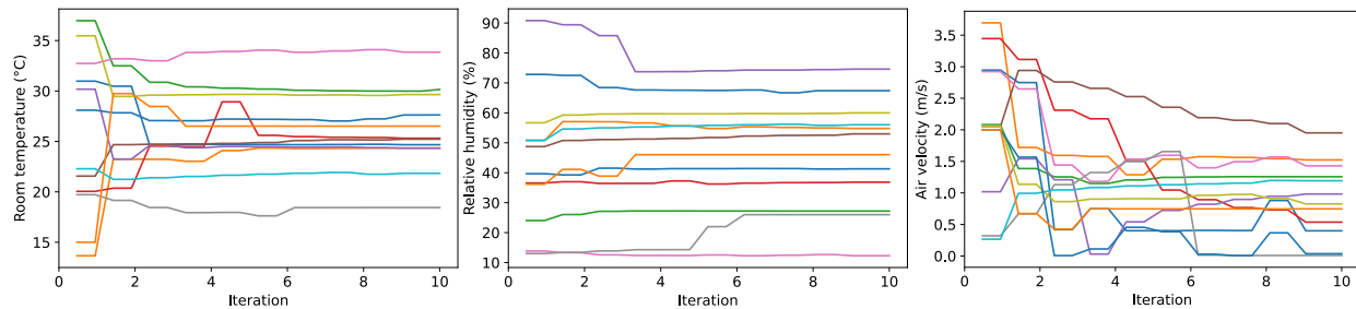
Figure 5: Changes in (a) air temperature, (b) relative humidity, and (c) air velocity during the optimization process.
