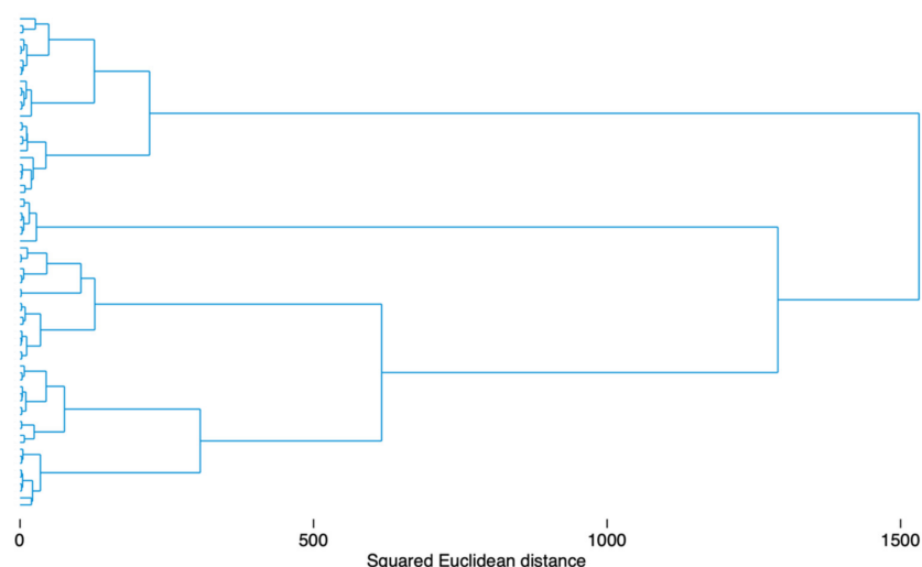
Figure 2. Dendrogram for the hierarchical cluster analysis.
