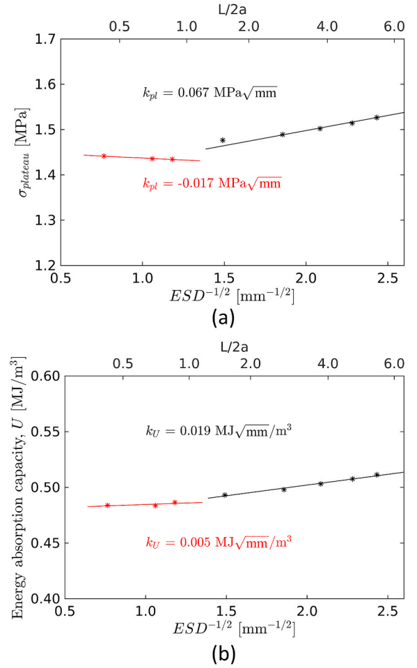
Fig. 11. Compressive properties for oxidized , Al-6101-T6 foam models: (a) plateau stress, \sigma_{plateau} , and (b) energy absorption capacity, U .
