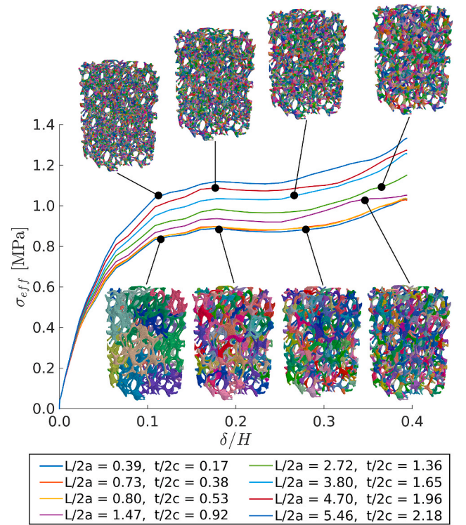
Fig. 8. Effective stress-strain responses of different grain-resolved, non-oxidized foam models. The average grain size is normalized by average geometric parameters of the struts to quantify the typical number of grains along the length ( L/2a ) and across the thickness ( t/2c ) of a nominal strut. The inset figures show the corresponding grain instantiations, depicted in an undeformed state.
