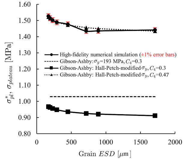
Fig. 13. Comparison between plateau stress based on high-fidelity numerical simulations and the plastic collapse strength based on the Gibson-Ashby formula versus average grain size for oxidized open-cell aluminum 6101-T6 foam. The Gibson-Ashby formula is evaluated using three different approaches for estimating \sigma_y and C_4 . Grain size is based on equivalent spherical diameter ( ESD ).
