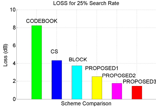
Fig. 7. Cost efficiency: Loss for fixed search rate.
