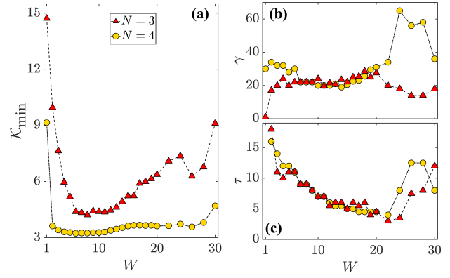
Figure 8: (a) Minimum of the kurtosis as a function of the number of wells for N = 3 (red triangles) and N = 4 (yellow circles). Kurtosis is calculated in an energy window of width \Delta E = 100 around E_{\text{mid}} = 700 . (b) Interaction and (c) barrier height corresponding to the points of minimum kurtosis in (a).
