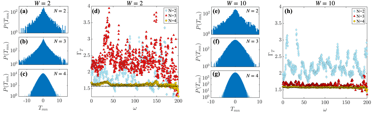
Figure 6: Off-diagonal elements of the kinetic energy operator T_{mn} for (a-d) W = 2 wells and (e-h) W = 10 wells. The probability distributions in the respective potentials are shown for (a,e) N = 2 (b,f) N = 3 and (c,g) N = 4 . (d,h) The ratio \Gamma_T as a function of \omega = |E_m - E_n| in an energy window at E_{\text{mid}} = 700 and width \Delta E = 100 . The interaction strengths and barrier heights are chosen at the point of minimum kurtosis for 4 particles in Fig.5(c,f), namely \gamma = 30 and \tau = 15 for W = 2 , and \gamma = 20 and \tau = 7.5 for W = 10 .
