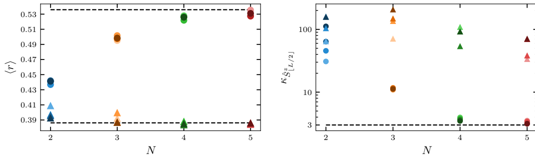
Figure 1: Left panel: Quantum chaos indicator \langle r \rangle as a function of the number of excitations N calculated for the integrable model \hat{H}_\infty^0 ( \blacktriangle ) and the single-impurity model \hat{H}_\infty^{\text{imp}} ( \bullet ). Right panel: same as the left panel, but for the kurtosis \kappa of the distribution of the off-diagonal elements of the middle-site magnetization. Each color represents a number of excitations with the darker shades corresponding to larger system sizes. The system sizes ranges used are: N = 2, L \in [100, 200] ; N = 3, L \in [30, 50] ; N = 4, L \in [22, 28] and N = 5, L \in [16, 21] .
