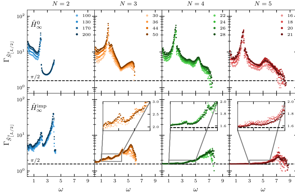
Figure 3: Ratios \Gamma_{\hat{S}_{[L/2]}^z}^z(\omega) for the integrable model \hat{H}_\infty^0 (top row) and the single-impurity model \hat{H}_\infty^{\text{imp}} (bottom row) for different number of excitations (different columns). In each panel, larger system sizes are represented by darker colors (see legends). The insets zoom in into areas of interest and are on a linear scale. See main text for the explanation of how \Gamma_{\hat{S}_{[L/2]}^z}^z(\omega) was calculated.
